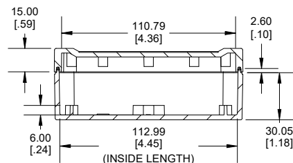
SECTION A-A SIDE VIEW
