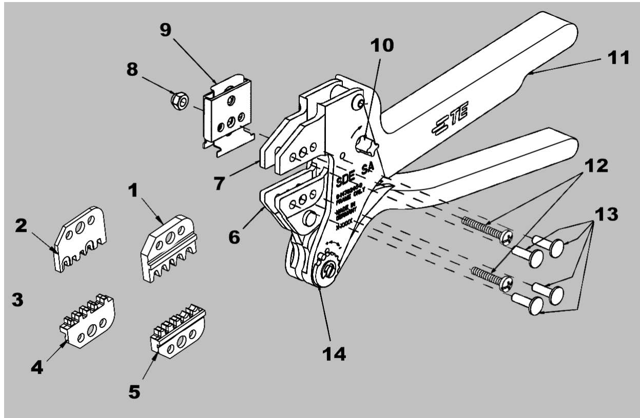
Figure 1: SDE-SA Commercial Hand Tool Assembly 2063524-1 with Die Assembly 2063524-2
