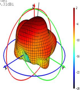
Phi=0 Freq=2350MHz
