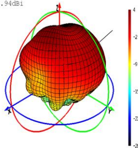
Phi=0 Freq=2140MHz
