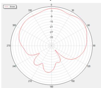
Phi=0 Freq=2600MHz
