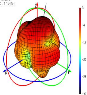
Phi=0 Freq=2140MHz
