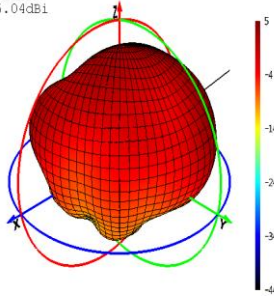
Phi=0 Freq=2350MHz
