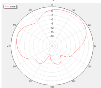
Phi=90 Freq=2140MHz
