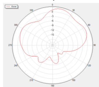
Phi=90 Freq=2350MHz
