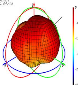
2600 MHz
