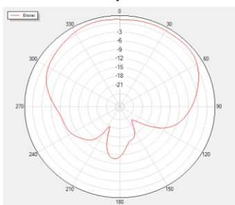
Phi=0 Freq=2350MHz
