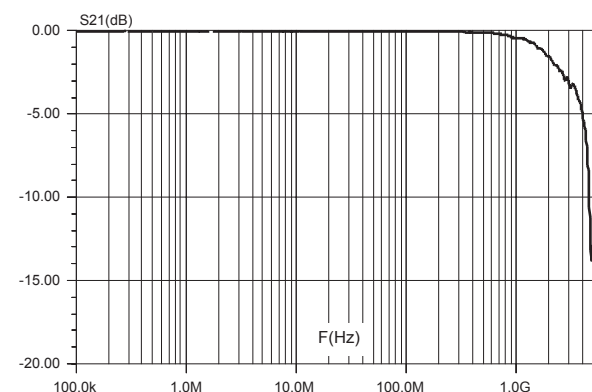
Figure 4. Frequency response
