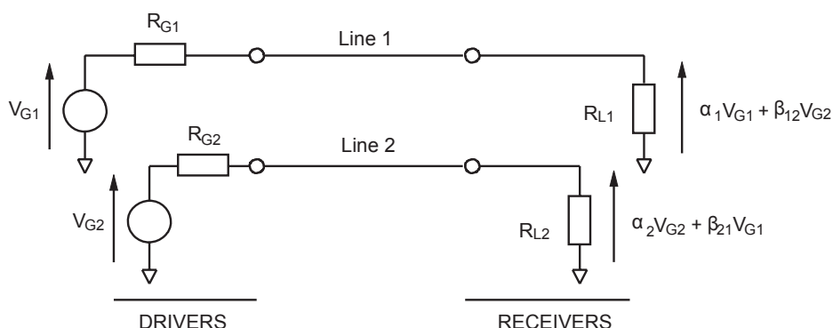
Figure 10. Crosstalk phenomenon
