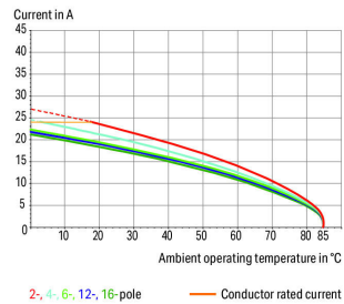
Derating Curve 2-conductor female connector (231-2102/026-000) with THT male header (231-132/001-000) Pin spacing: 5 mm / Conductor cross-section: 2.5 mm 2 "F-st" Based on: EN 60512-5-2 / Reduction factor: 0.8
