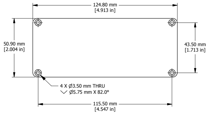
END PLATE
