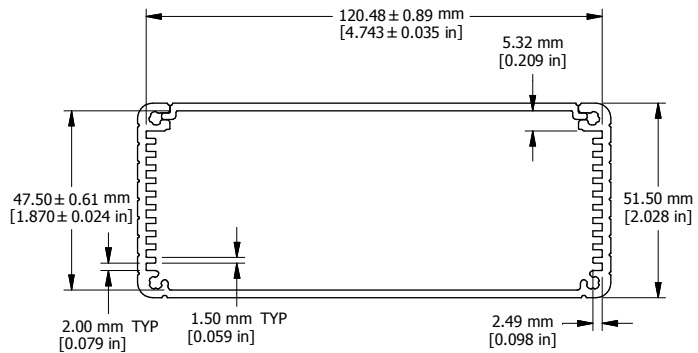
EXTRUSION
