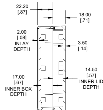
SECTION B-B SIDE VIEW
