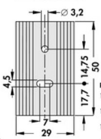
SK 09 50 TO 220
