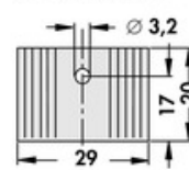
SK 09 20 TO 220
