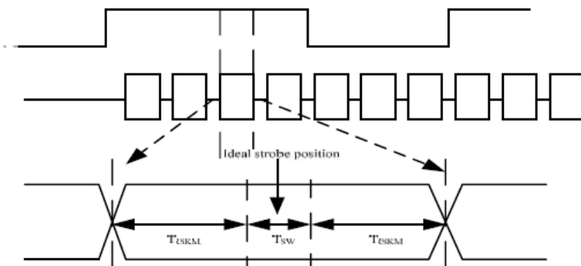
LVDS timing(2)
