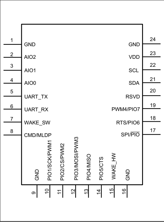
FIGURE 1-2: RN4020 PIN DIAGRAM
