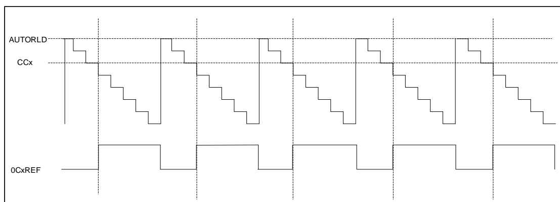
Figure 65 PWM1 Count-down Mode Timing Diagram
