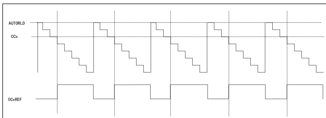
Figure 75 PWM1 Count-down Mode Timing Diagram
