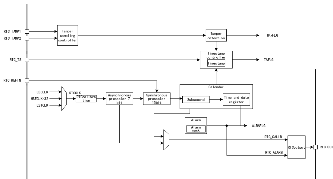
Figure 92 APM32F030x4x6x8 RTC Structure Block Diagram
