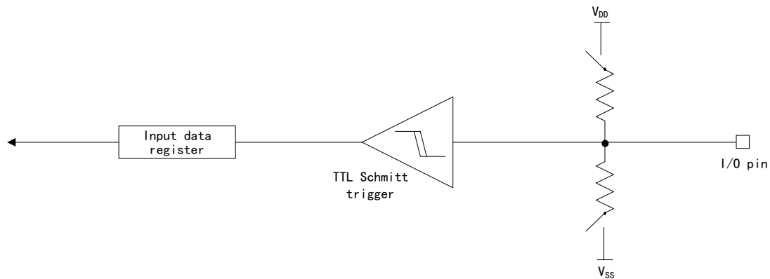
Figure 17 I/O Structure in Input Mode Read
