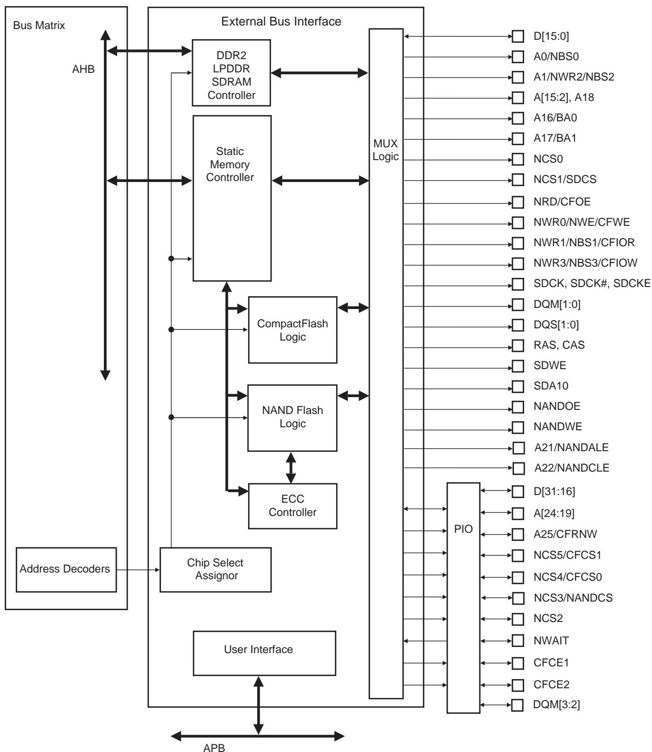
Figure 19-3. Organization of the External Bus Interface
