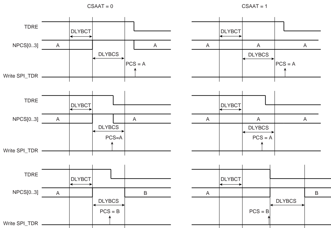
Figure 29-12. Peripheral Deselection
