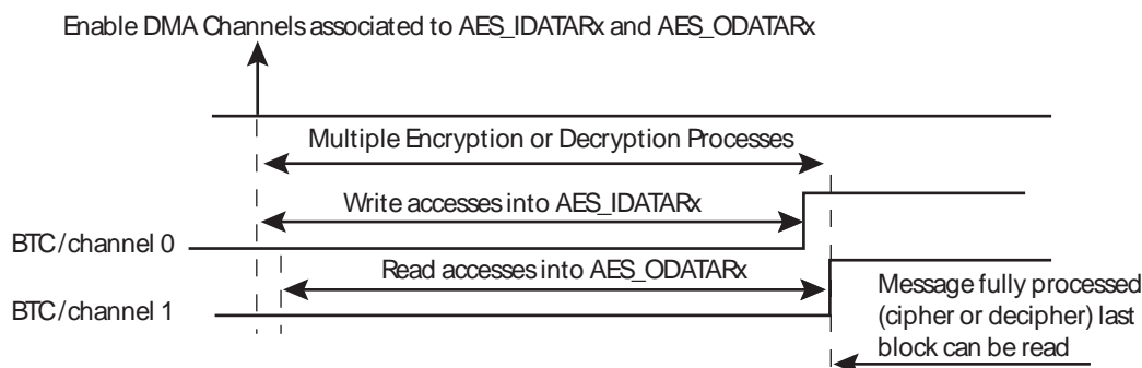
Figure 43-3. DMA transfer with LOD = 0
