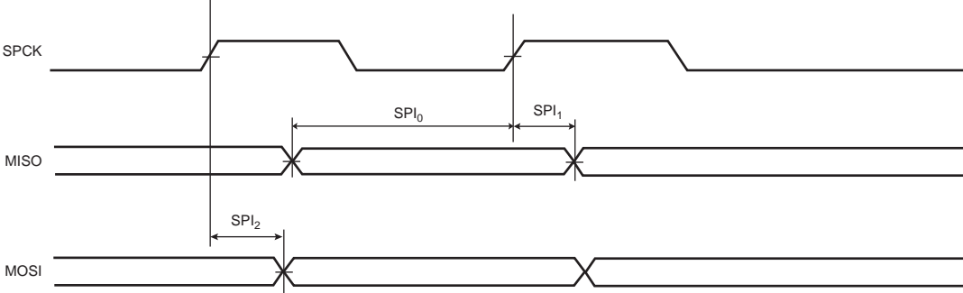
Figure 49-5. SPI Master Mode 1 and 2
