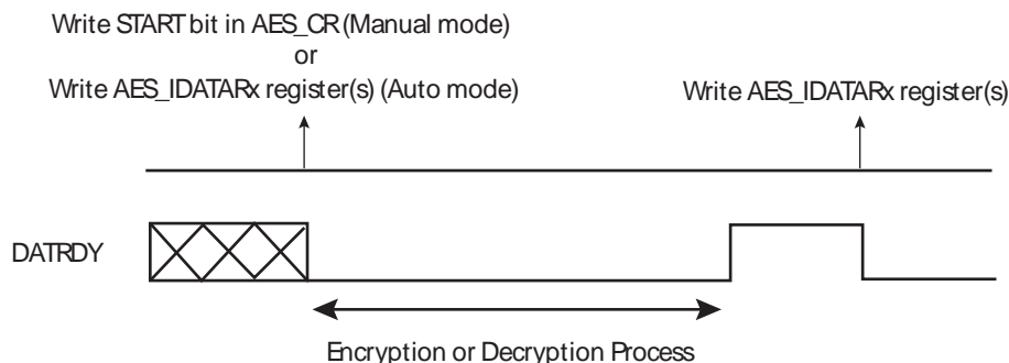
Figure 43-2. Manual and Auto Modes with LOD = 1
