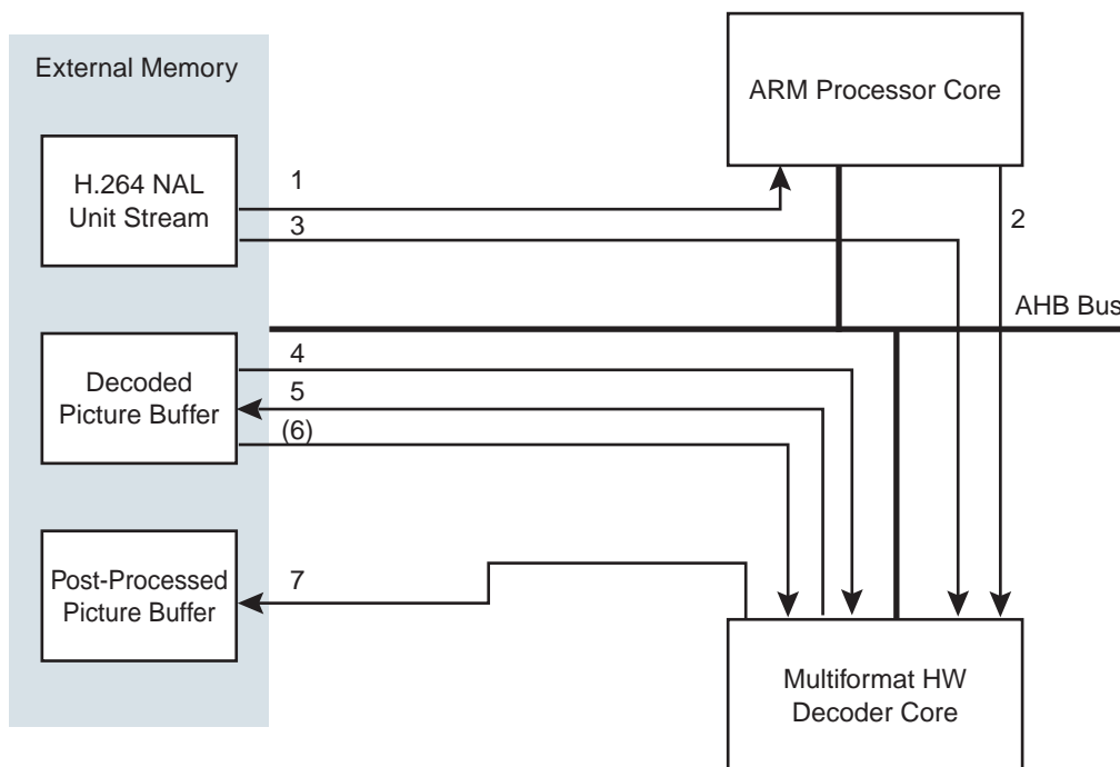
Figure 47-2. Multi-format Decoder and External Memory Data Flow in VLC Mode
