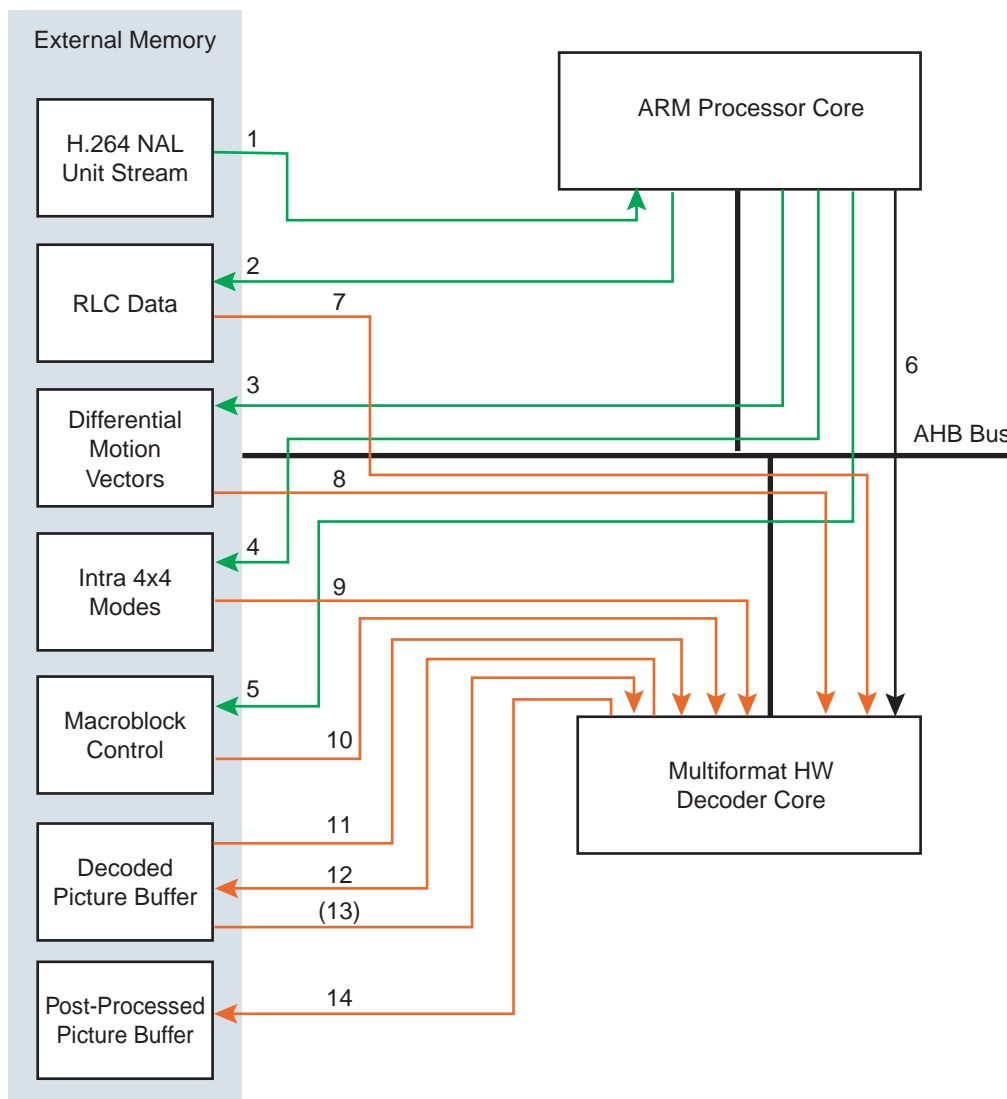
Figure 47-3. Multi-format Decoder and External Memory Data Flow in RLC Mode
