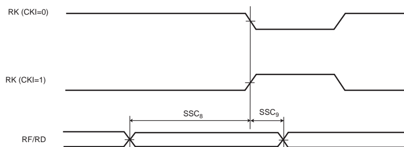
Figure 49-14. SSC Receiver RK and RF in Input
