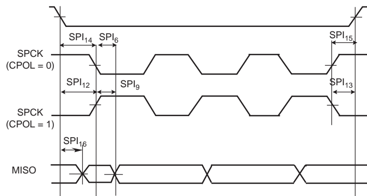
Figure 49-25. SPI Slave Mode - NPCS Timings
