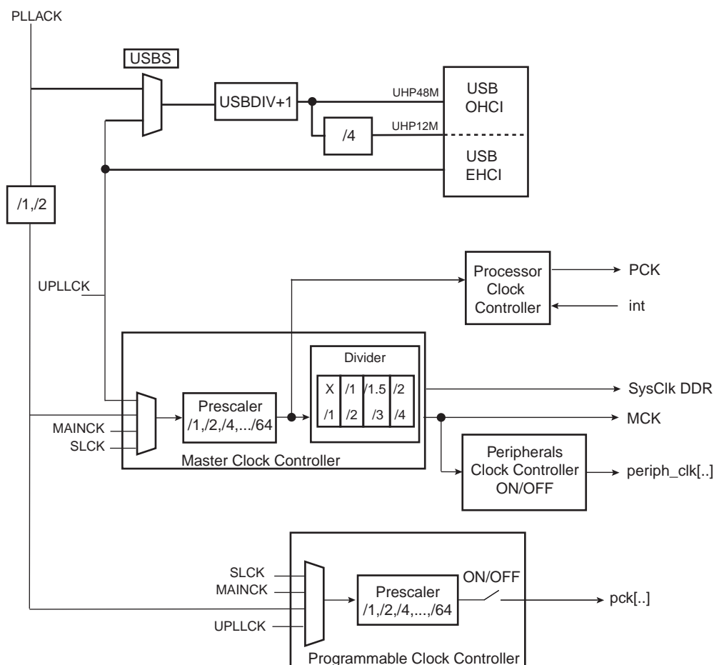
Figure 25-1. SAM9M11 Power Management Controller Block Diagram
