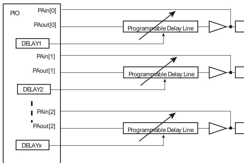
Figure 28-7. Programmable I/O Delays
