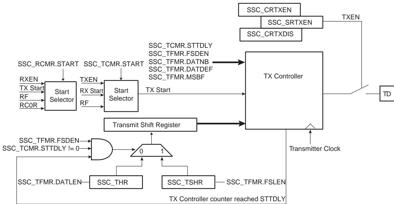
Figure 35-9. Transmitter Block Diagram
