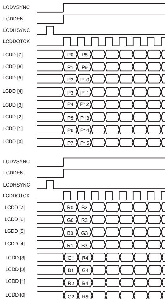
Figure 48-10. Single Scan Monochrome and Color 8-bit Panel Timing (First Line Expanded View)
