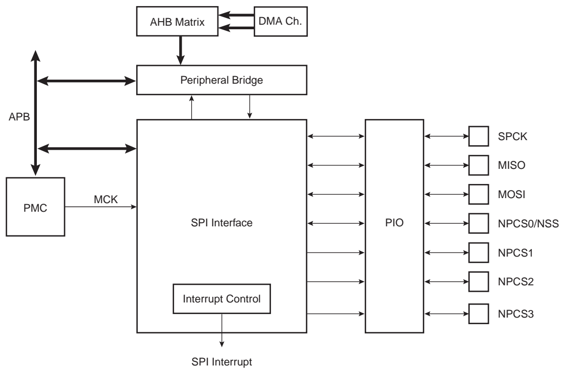
Figure 29-2. Block Diagram
