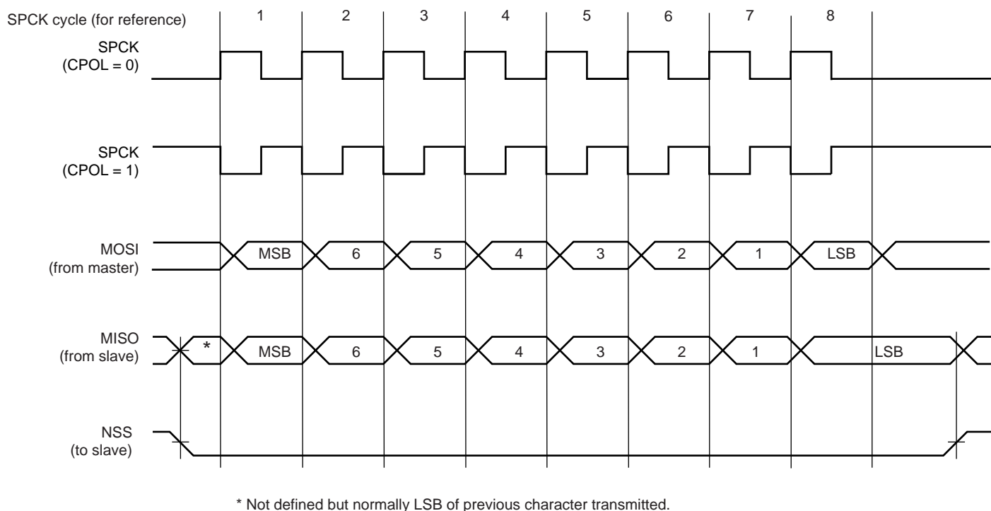
Figure 29-5. SPI Transfer Format (NCPHA = 0, 8 bits per transfer)
