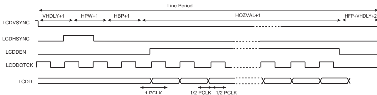
Figure 48-7. TFT Panel Timing (Line Expanded View), CLKMOD = 1
