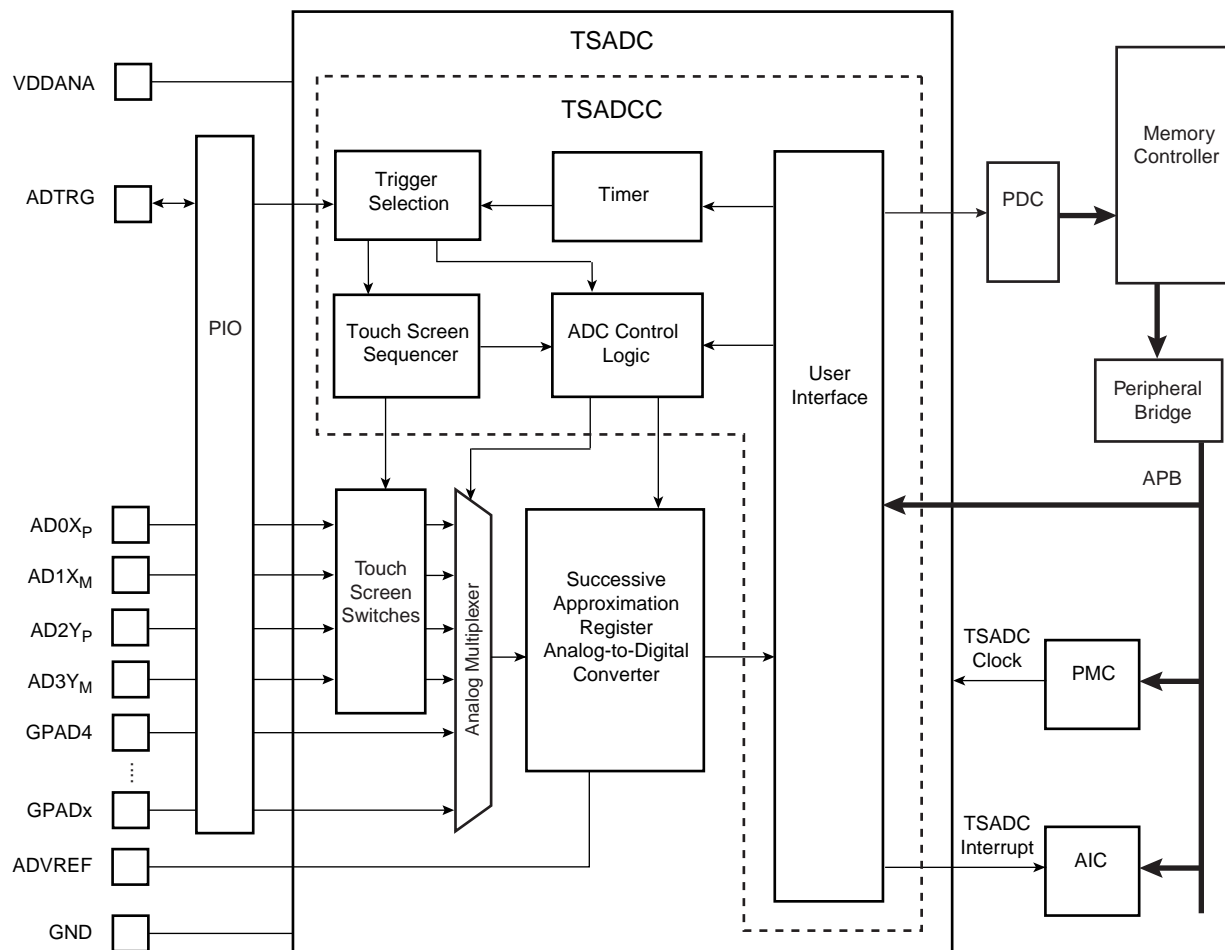
Figure 41-1. TSADCC Block Diagram
