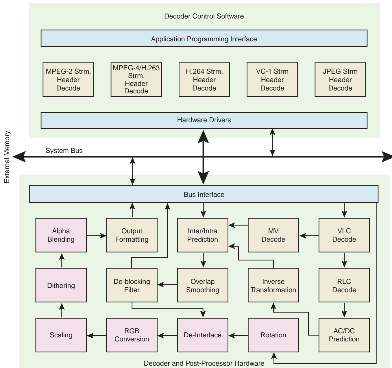
Figure 47-1. Block Diagram
