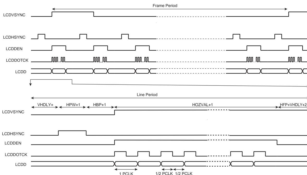
Figure 48-5. STN Panel Timing, CLKMOD 0
