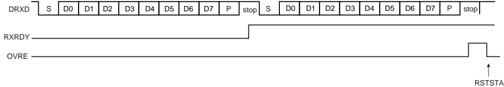
Figure 27-7. Receiver Overrun
