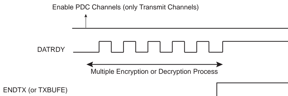
Figure 44-4. PDC Mode with LOD = 1
