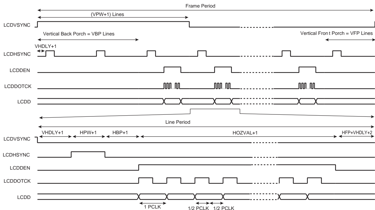
Figure 48-6. TFT Panel Timing, CLKMOD = 0, VPW = 2, VBP = 2, VFP = 1
