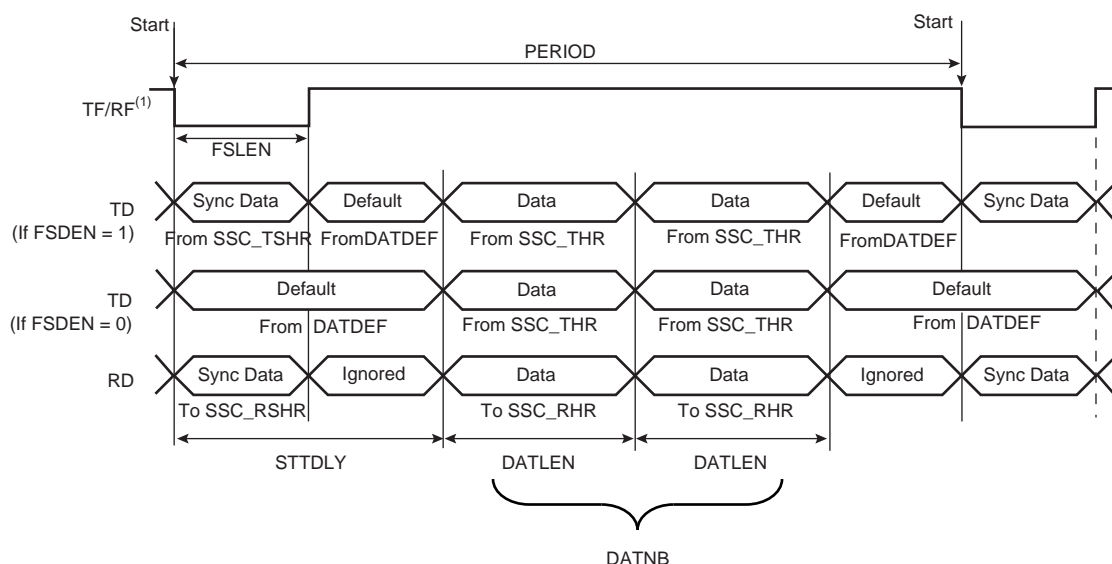
Figure 35-14. Transmit and Receive Frame Format in Edge/Pulse Start Modes
