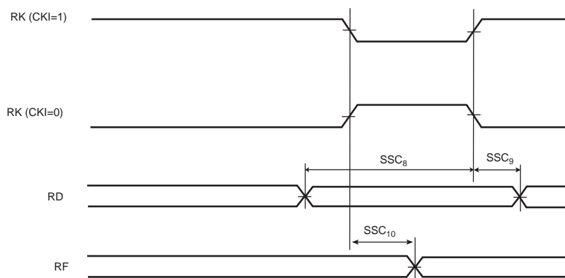
Figure 49-15. SSC Receiver, RK in Input and RF in Output
