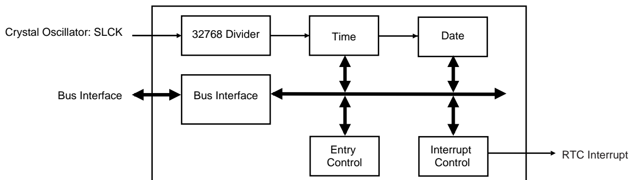
Figure 12-1. RTC Block Diagram
