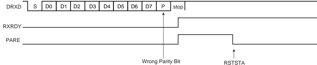
Figure 27-8. Parity Error
