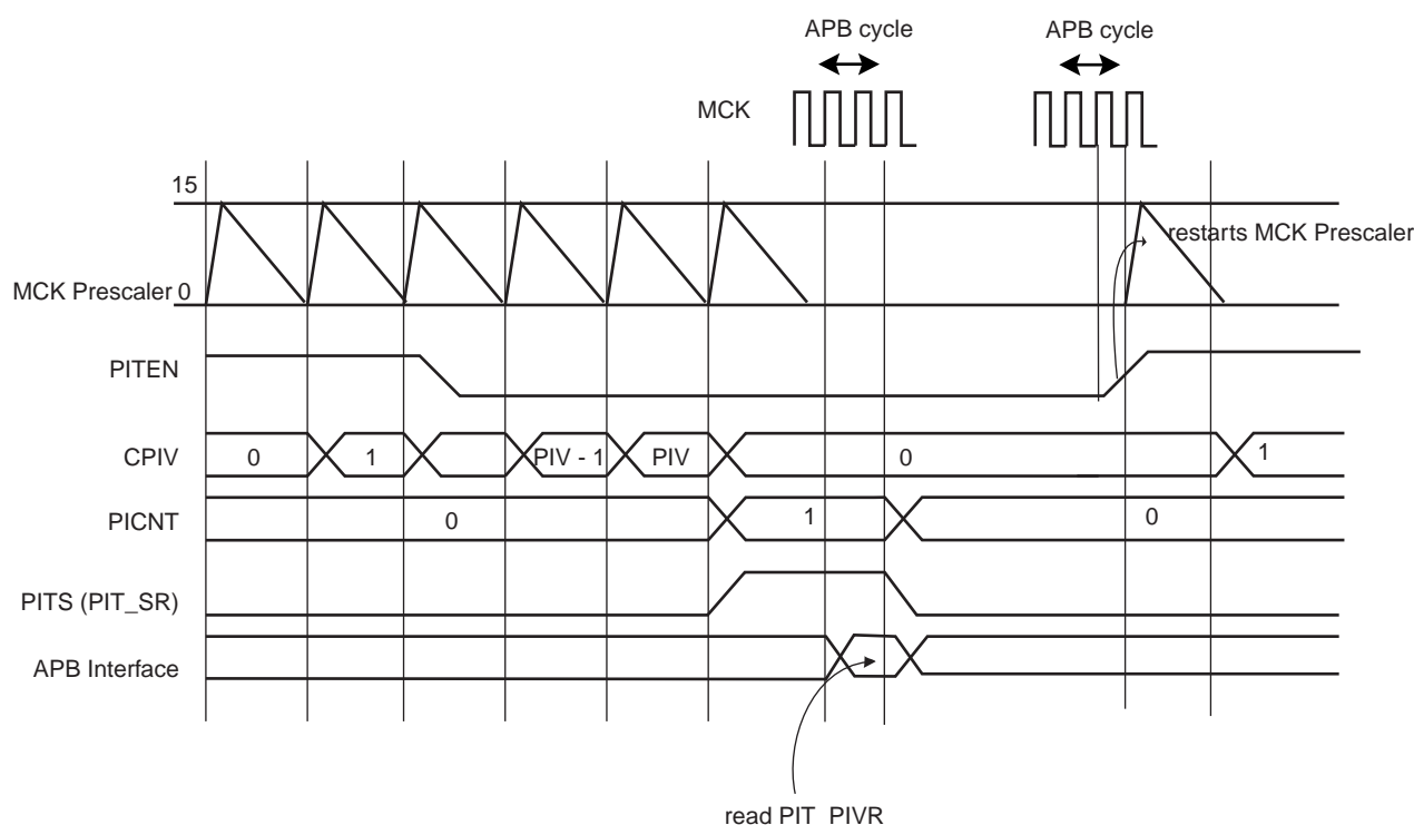
Figure 14-2. Enabling/Disabling PIT with PITEN
