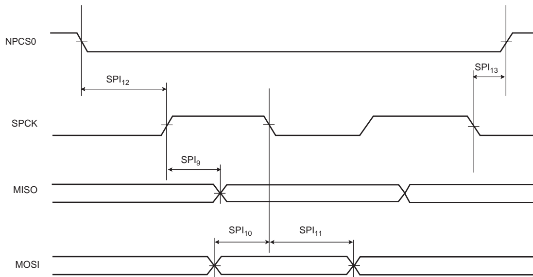
Figure 49-8. SPI Slave Mode 1 and 2
