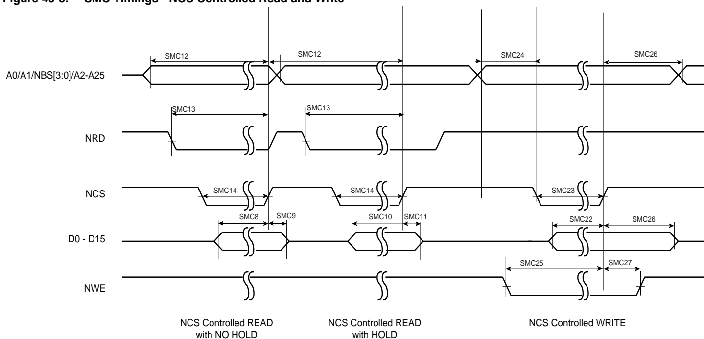
Figure 49-3. SMC Timings - NCS Controlled Read and Write
