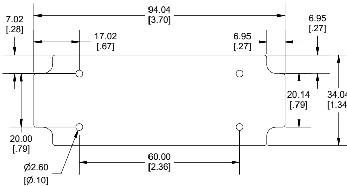
MAXIMUM P.C. BOARD SIZE
