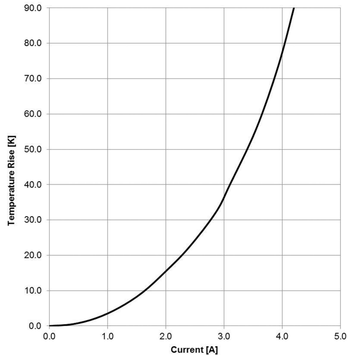
F2 Typical Temperature Rise vs. Current Characteristics:
