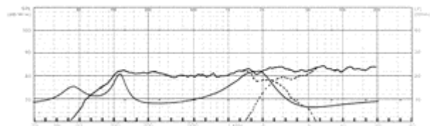
Frequency response
