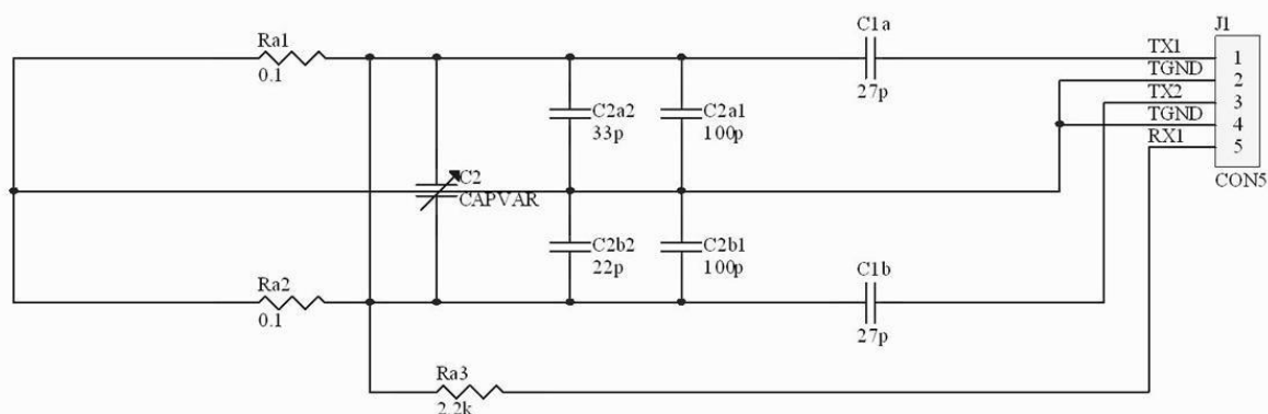
External Antenna Circuit Diagram detail
