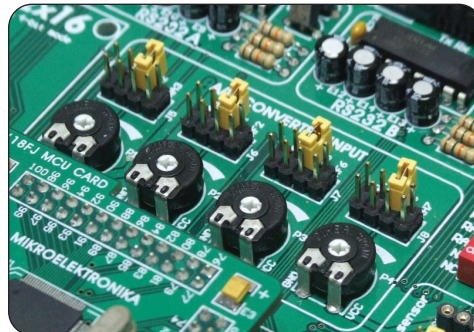
A/D Converter Figure 32.
