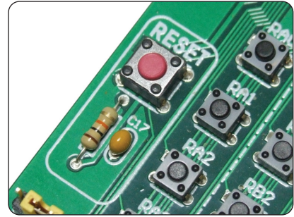
Reset switch Figure 16.
