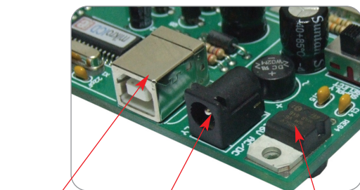
USB connector
