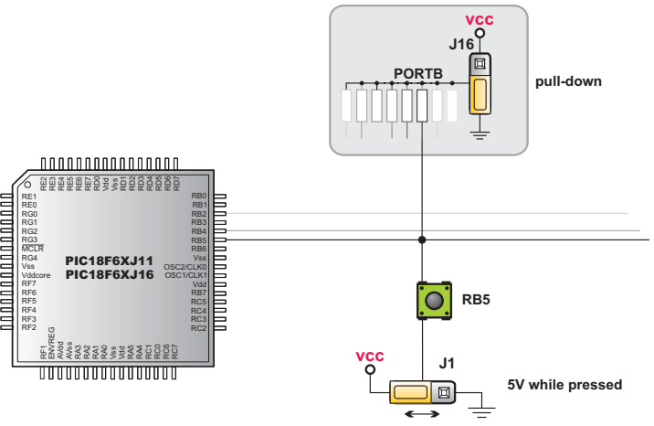
Figure 21. Button with pull-down resistor
