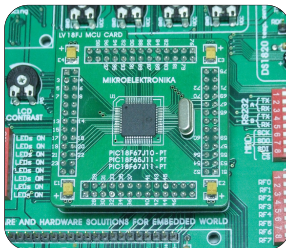
Figure 6. MCU placed on socket
