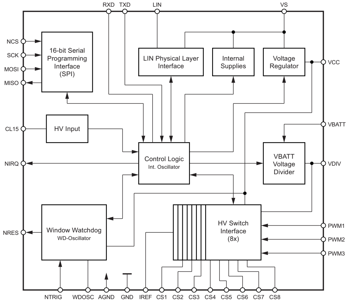
Figure 4-1. Block Diagram
