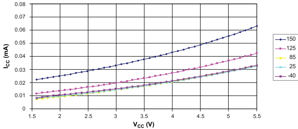
Figure 5-121. Idle Supply Current versus V_{CC} (Internal RC Oscillator, 128kHz)
