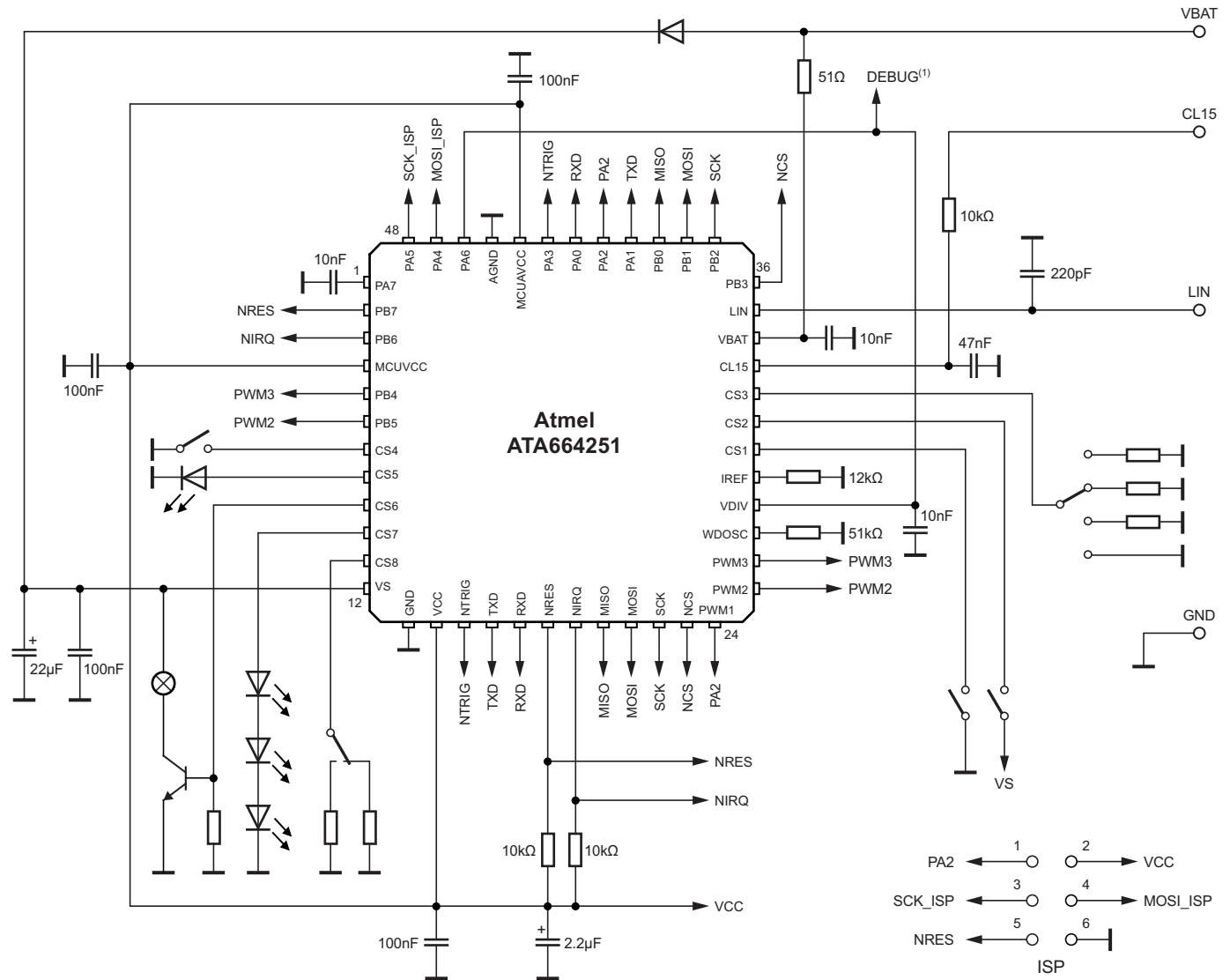
Figure 6-1. Application Example 1: LIN Slave with Different External Circuitry at the CSx-pins
