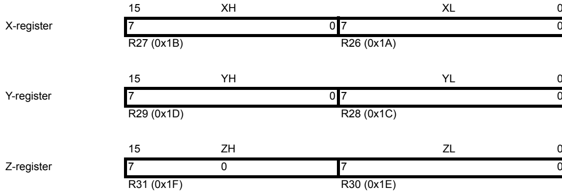
Figure 5-4. The X-, Y-, and Z-registers
