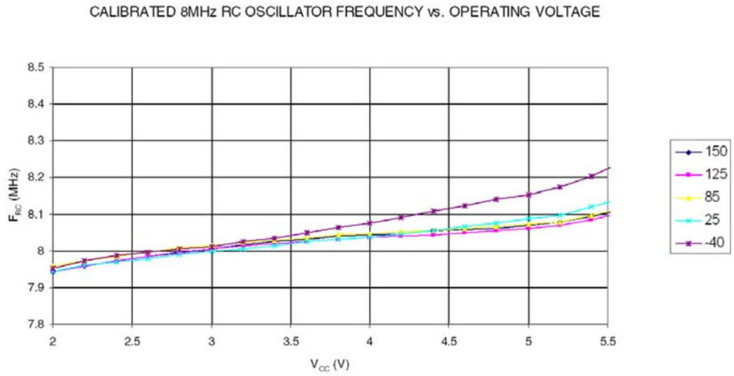
Figure 5-132. Calibrated 8.0MHz RC Oscillator Frequency versus V CC
