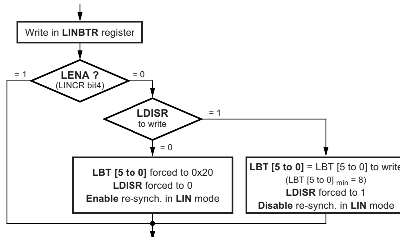
Figure 5-75. Handling LBT[5..0]
