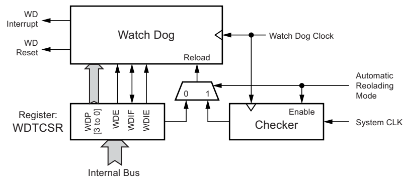
Figure 5-15. Watchdog Timer with Automatic Reloading
