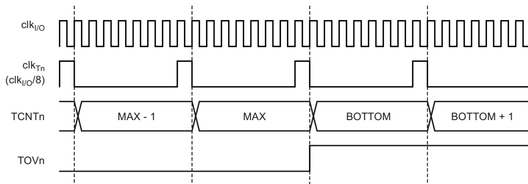
Figure 5-38. Timer/Counter Timing Diagram, with Prescaler ( f_{\text{clk\_I/O}}/8 )
