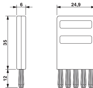
Dimensional drawing
