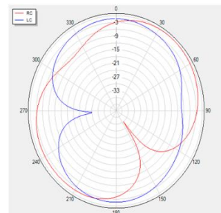
Theta=90 freq=1602MHz
