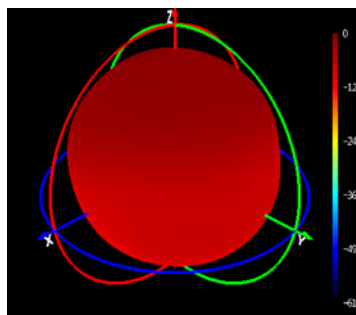
Phi=90 freq=1575MHz
