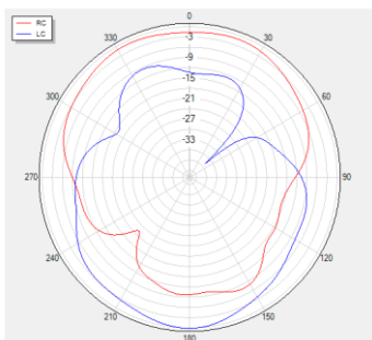
Phi=90 freq=1176MHz
