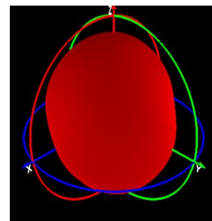
Phi=90 freq=1602MHz
