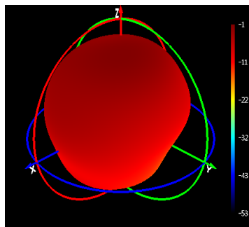
Phi=90 freq=1176MHz
