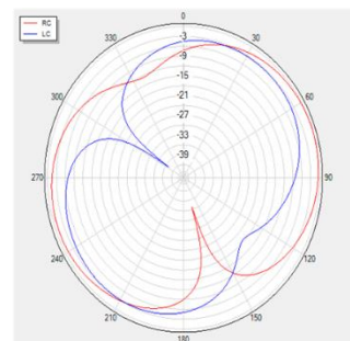
Theta=90 freq=1561MHz
