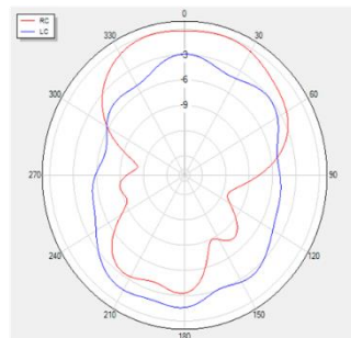
Phi=0 freq=1561MHz
