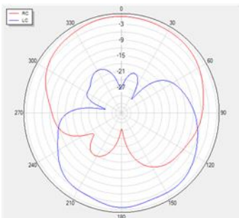
Phi=0 freq=1575MHz
