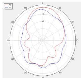
Phi=0 freq=1602MHz
