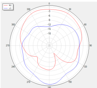
Phi=0 freq=1176MHz
