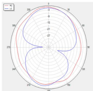
Phi=90 freq=1602MHz
