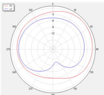
Theta=90 freq=1575MHz
