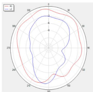
Phi=90 freq=1561MHz
