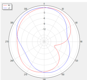
Theta=90 freq=1176MHz
