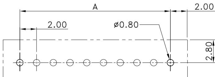
Recommended PCB Layout General Tolerances ±0.05
