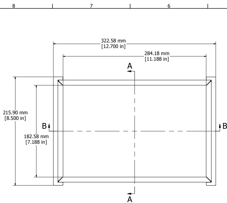
Assembly - View From Bottom
