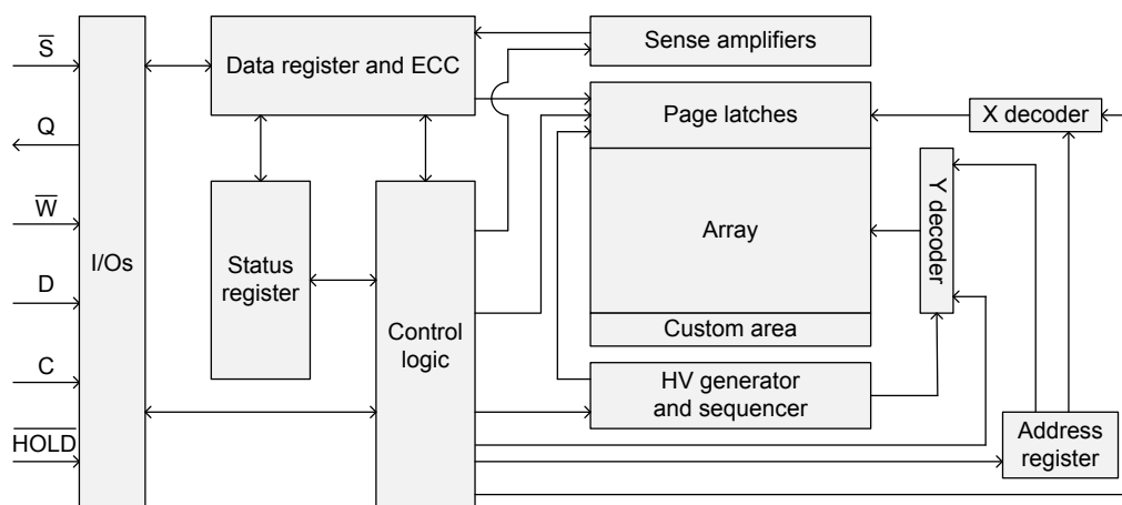
Figure 4. Block diagram
