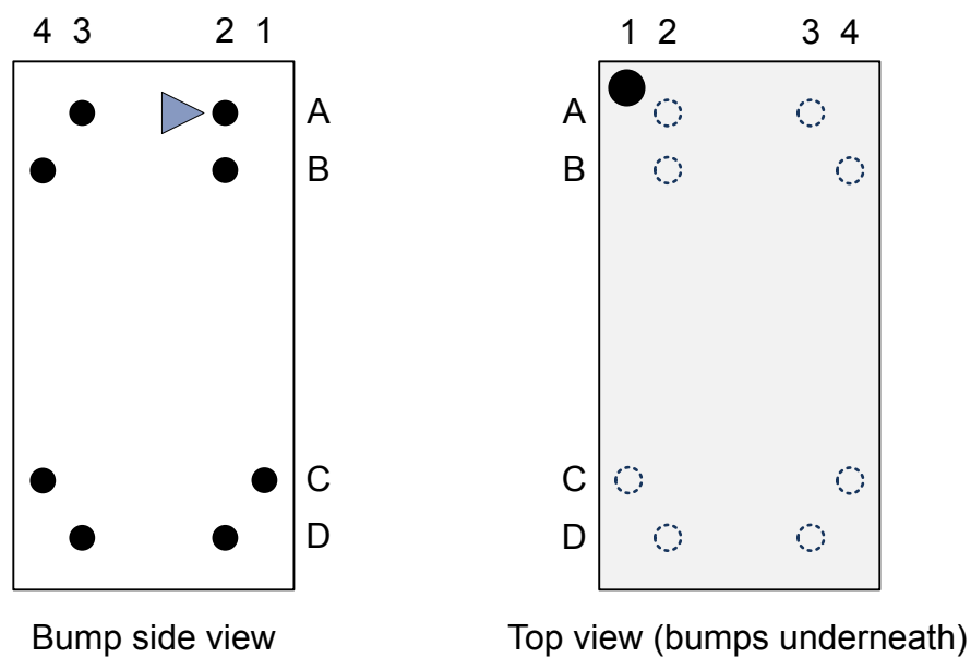
Figure 3. WLCSP connections
