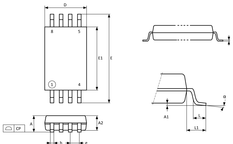
Figure 27. TSSOP8 – Outline
