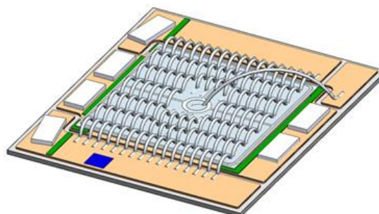
Power hybrid (example)
