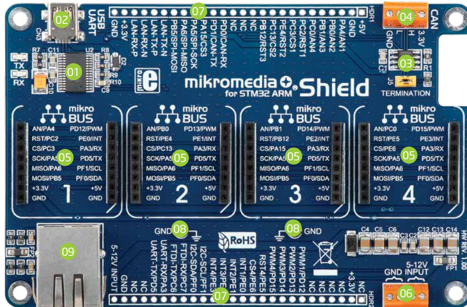
Figure 18-1: mikromedia+ shield
