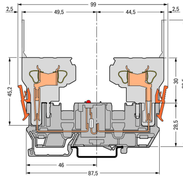
LED carrier terminal block
