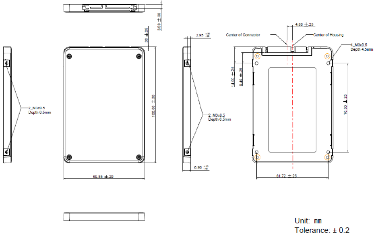
Figure 6-1 7mm Housing Physical Dimensions
