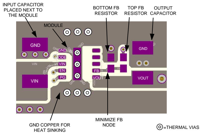
Figure 71. Layout Example With Adjustable Output Version
