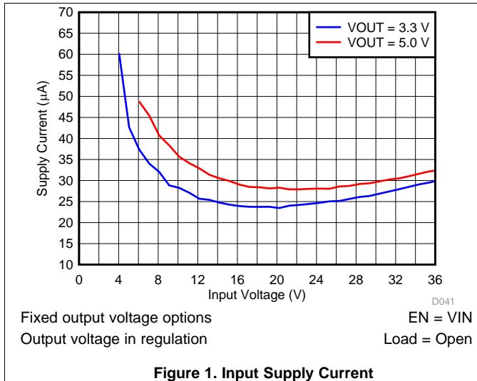
Figure 1. Input Supply Current
