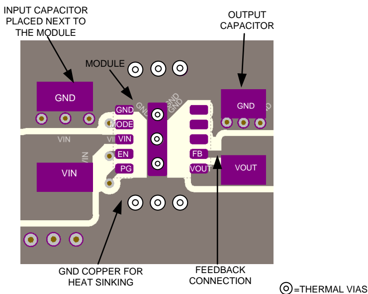
Figure 70. Layout Example With Fixed Output Version
