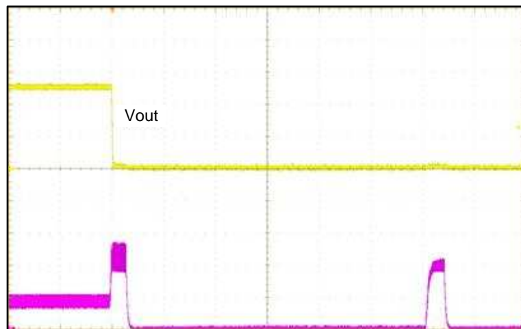
Figure 28. Hiccup Operation
