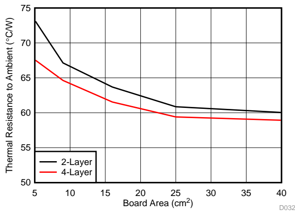
Figure 69. Package Thermal Resistance vs Board Copper Area
