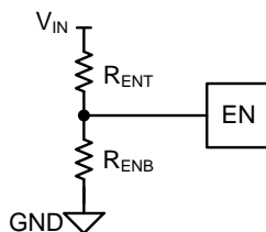
Figure 32. Enable Divider to Set External UVLO Threshold
