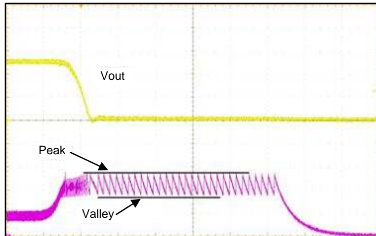
Figure 27. Current Limit Operation During Output Short Circuit
