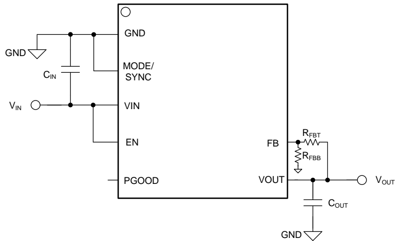
Figure 30. Adjustable 2.5-V to 15-V Output Typical Application Circuit
