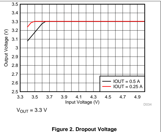
Figure 2. Dropout Voltage
