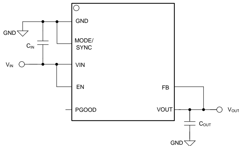
Figure 29. Fixed 5-V or 3.3-V Typical Application Circuit
