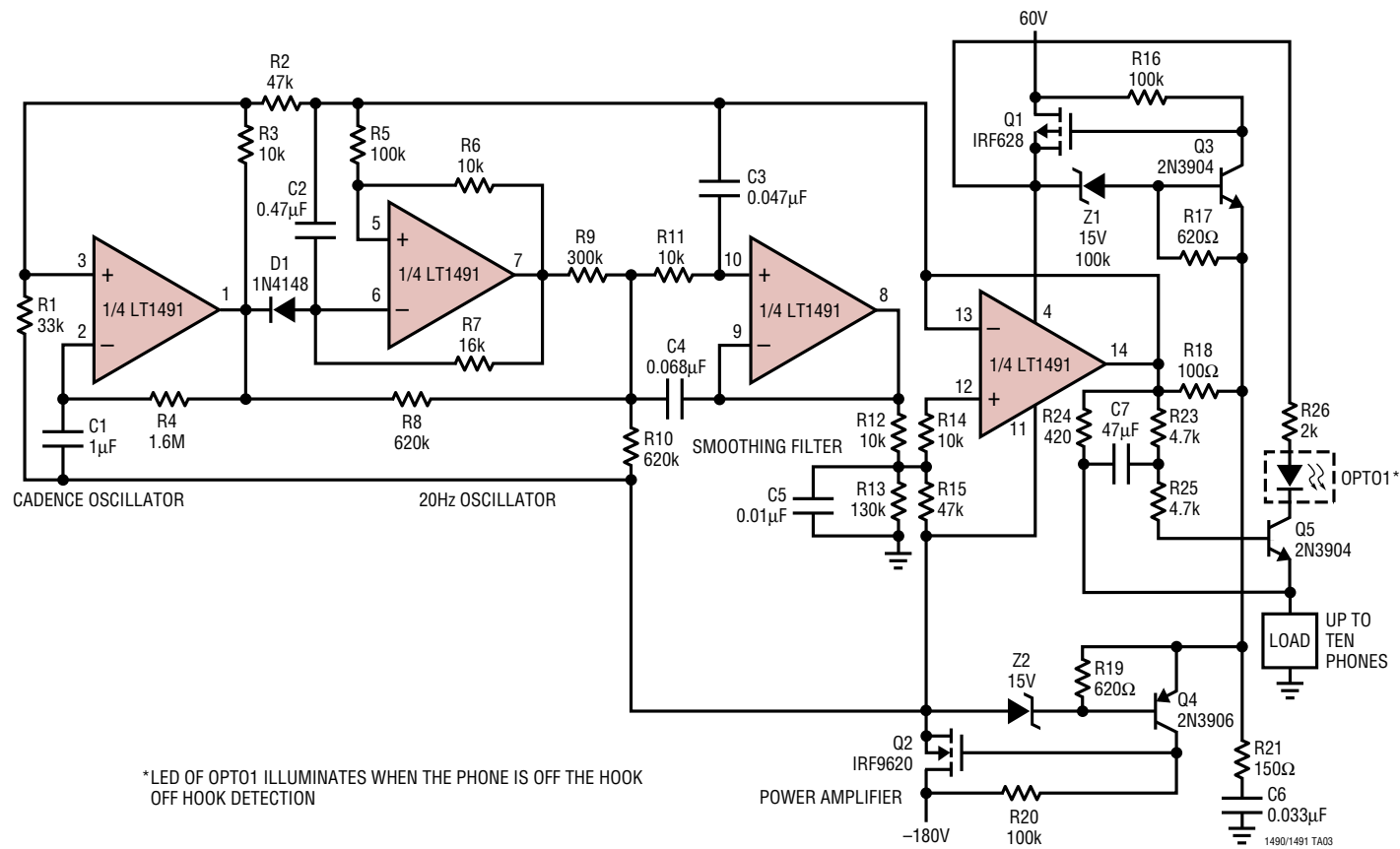
Ring-Tone Generator
