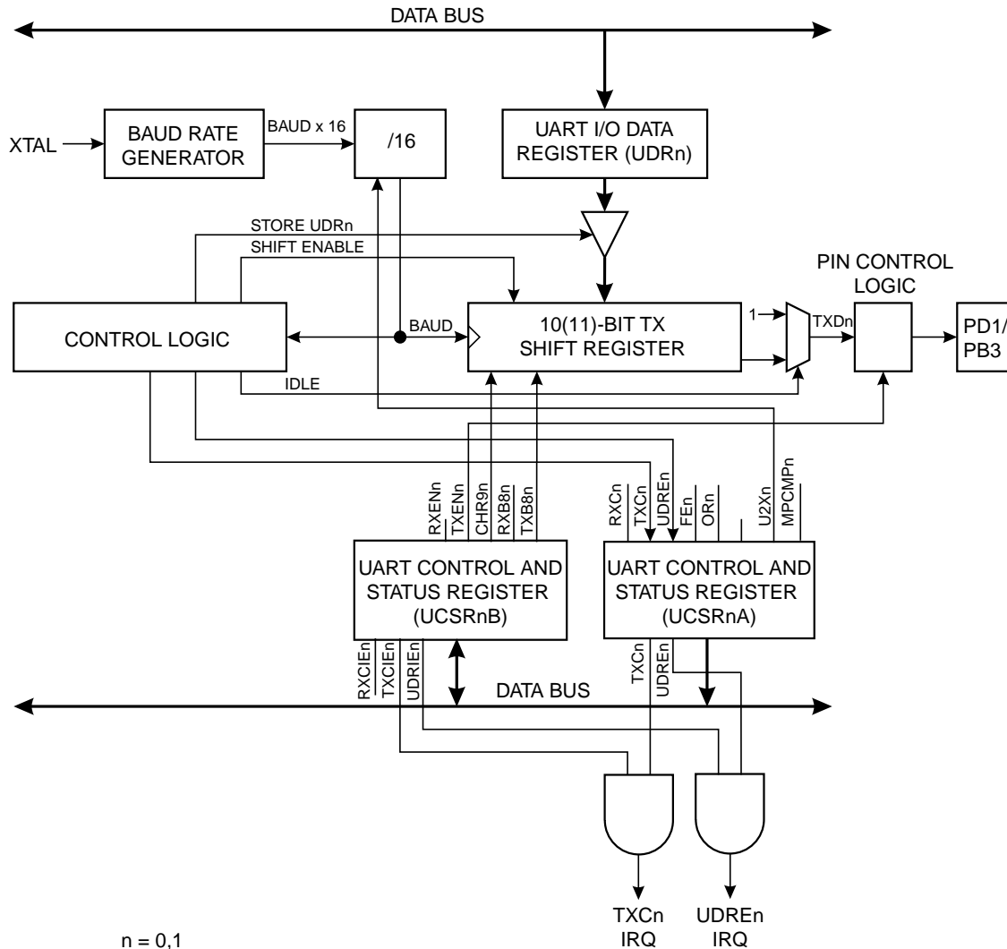
Figure 45. UART Transmitter
