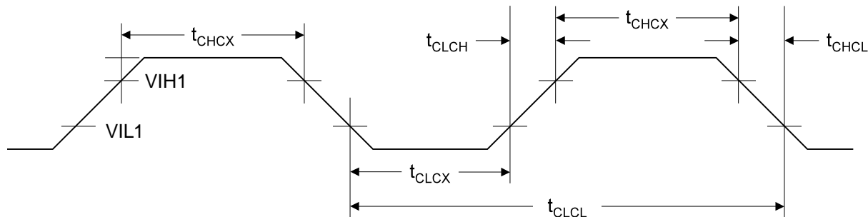
Figure 83. External Clock
