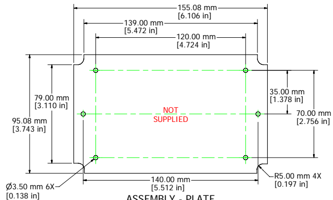
ASSEMBLY - PLATE
