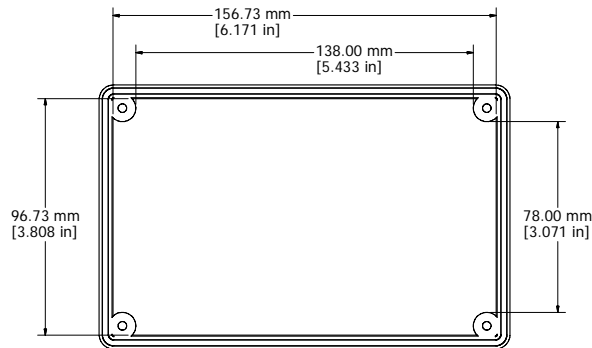
ASSEMBLY - INSIDE (LID)
