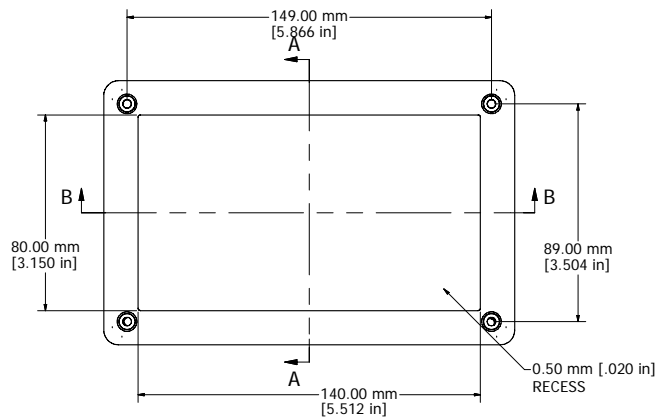
ASSEMBLY - TOP
