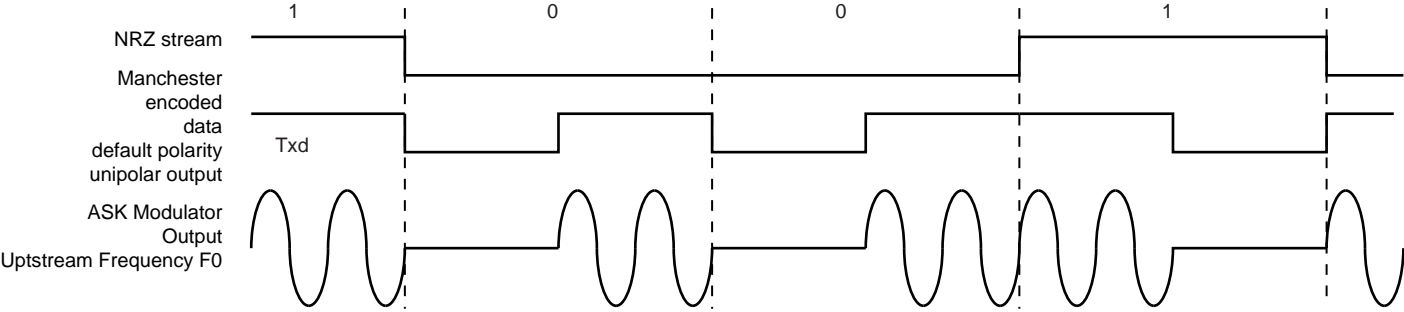
Figure 39-18.ASK Modulator Output
