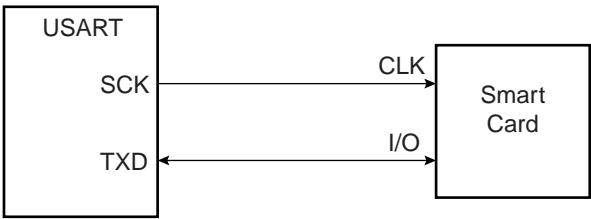
Figure 39-29.Connection of a Smart Card to the USART
