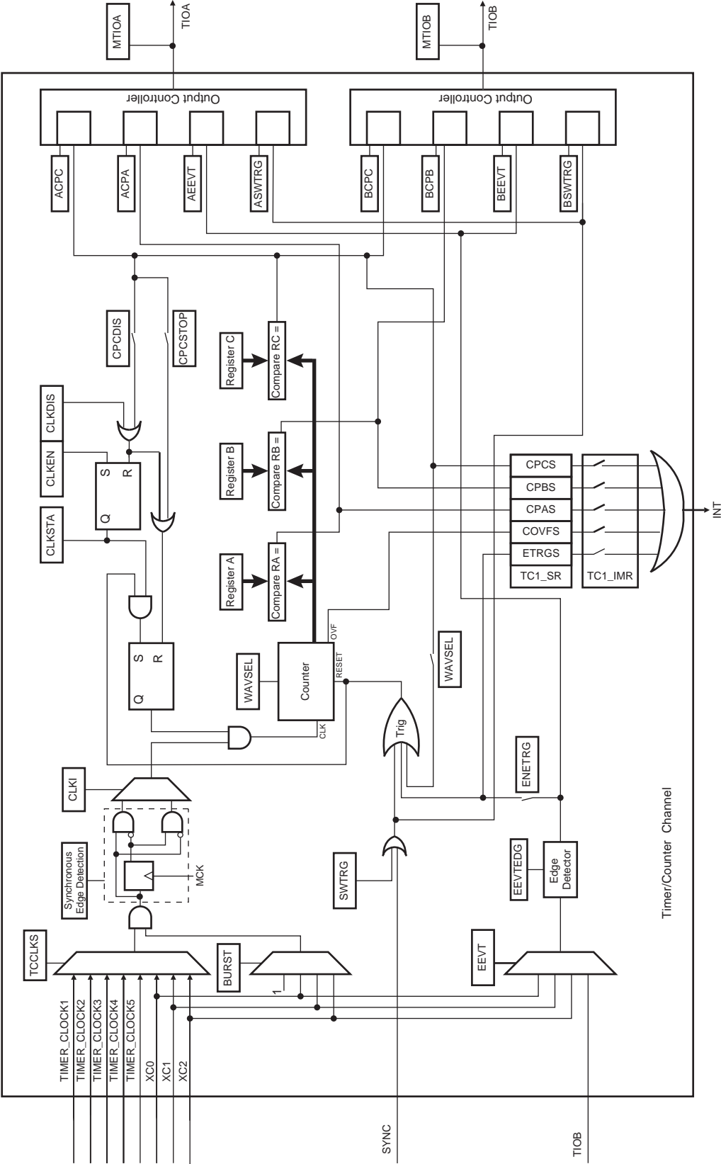
Figure 36-6. Waveform Mode
