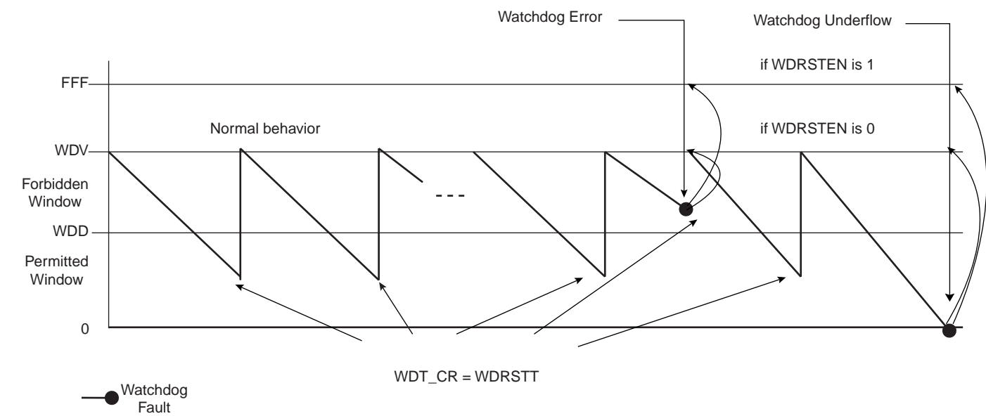
Figure 17-2. Watchdog Behavior
