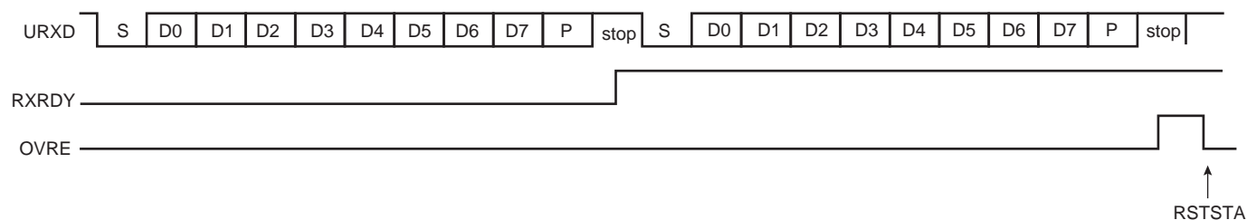
Figure 41-6. Receiver Overrun
