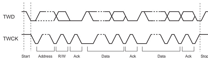
Figure 37-4. Transfer Format
