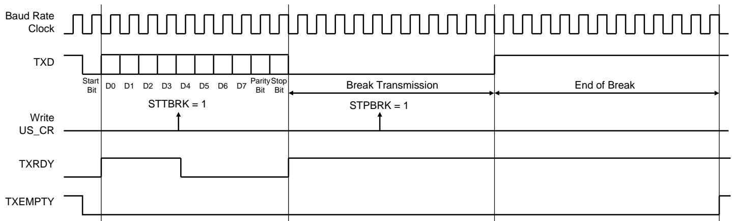
Figure 39-26. Break Transmission
