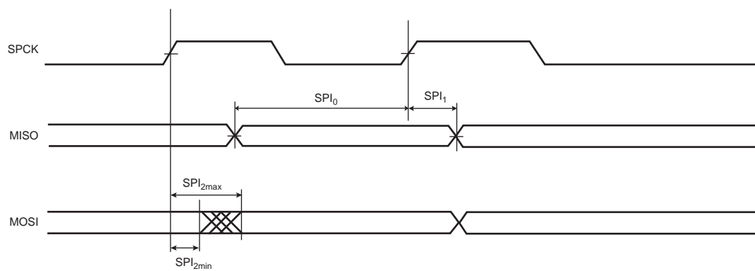
Figure 46-14. Min and Max access time for SPI output signal
