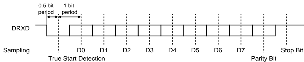
Figure 24-5. Character Reception Example: 8-bit, parity enabled 1 stop
