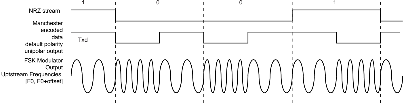
Figure 39-19.FSK Modulator Output
