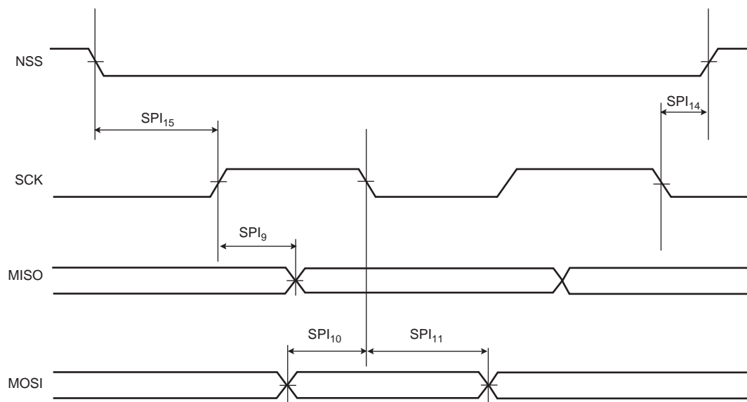
Figure 46-30.USART SPI Slave mode: (Mode 0 or 3)
