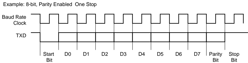
Figure 39-6. Character Transmit
