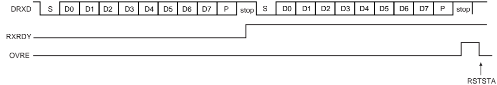
Figure 24-7. Receiver Overrun
