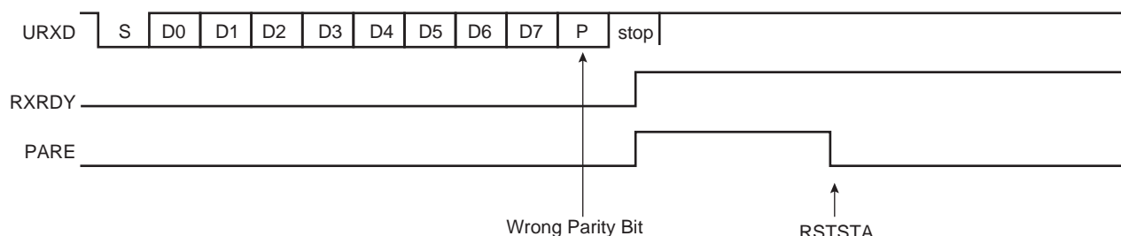
Figure 41-7. Parity Error
