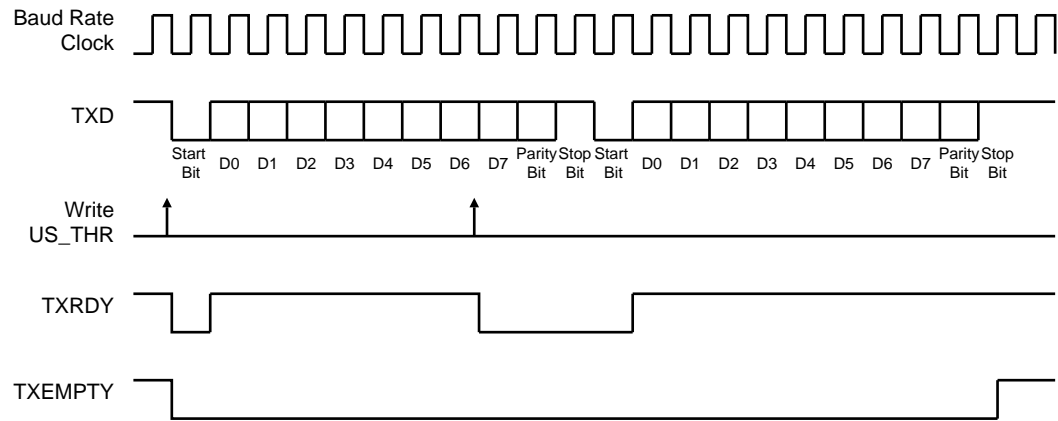
Figure 39-7. Transmitter Status
