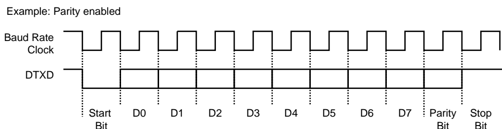
Figure 24-10.Character Transmission
