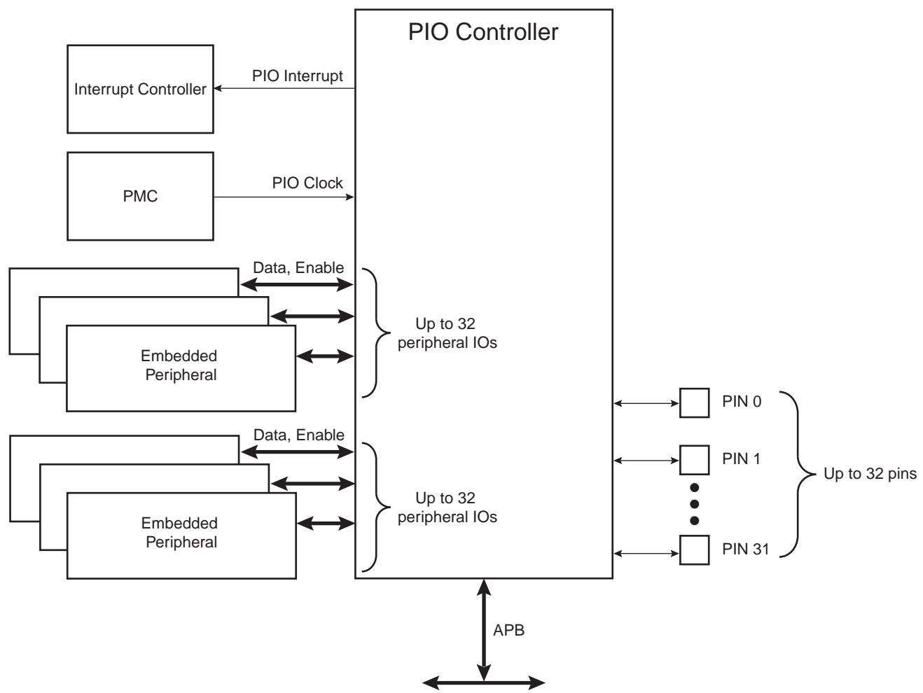
Figure 23-1. Block Diagram
