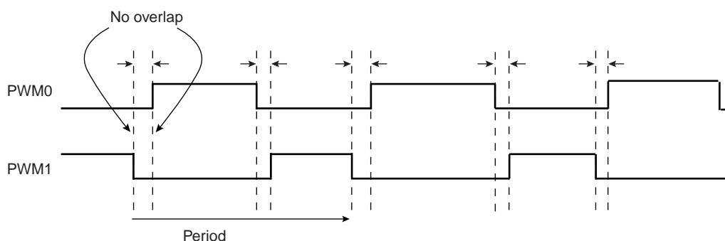
Figure 38-4. Non Overlapped Center Aligned Waveforms
