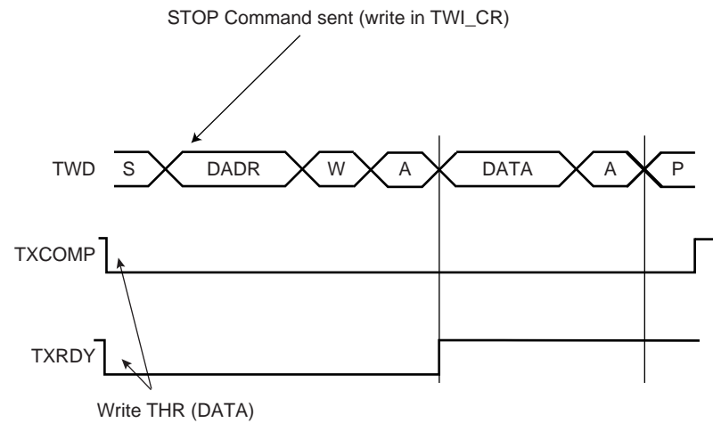
Figure 37-6. Master Write with One Data Byte
