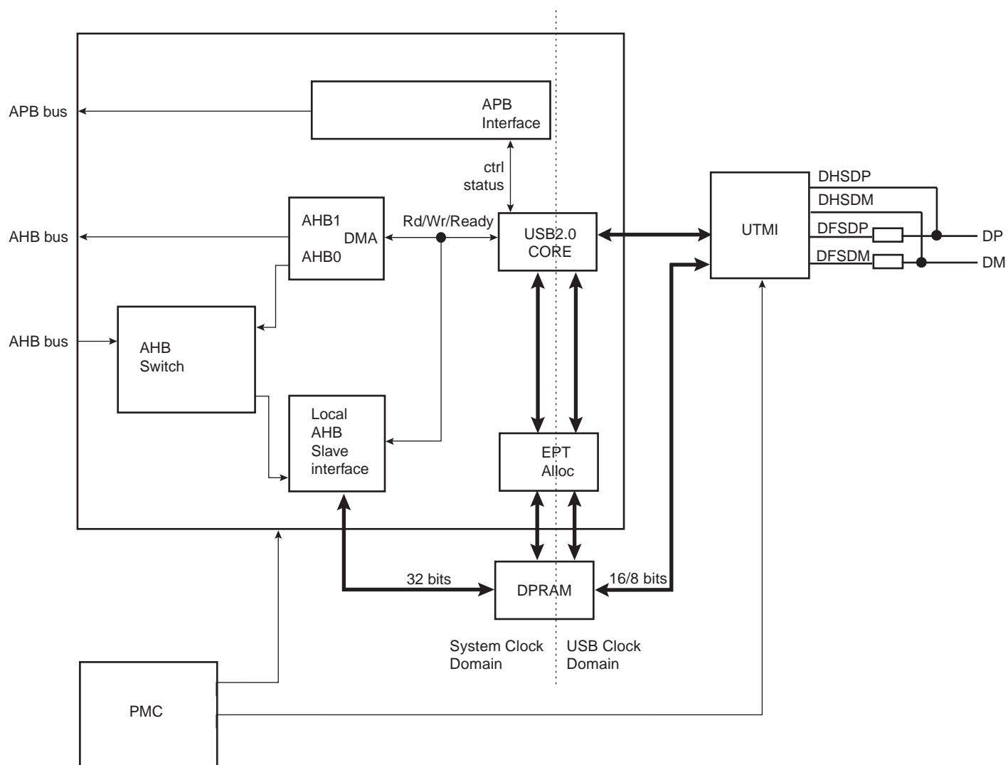
Figure 32-1. Block Diagram
