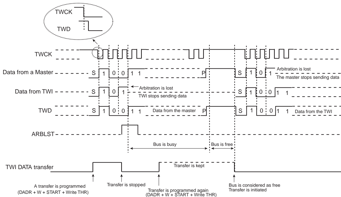
Figure 37-23. Arbitration Cases
