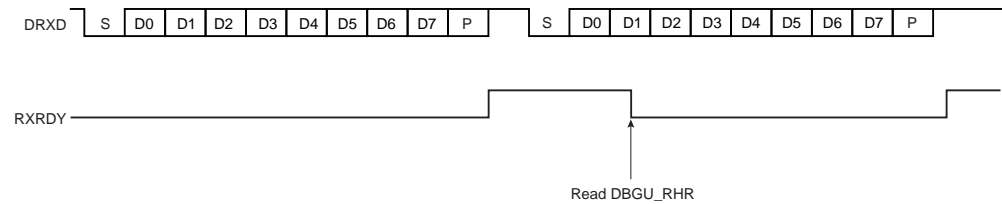
Figure 24-6. Receiver Ready
