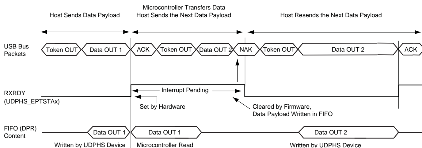
Figure 32-14.Data OUT Transfer for Endpoint with One Bank
