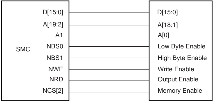
Figure 29-4. Memory Connection for a 16-bit Data Bus
