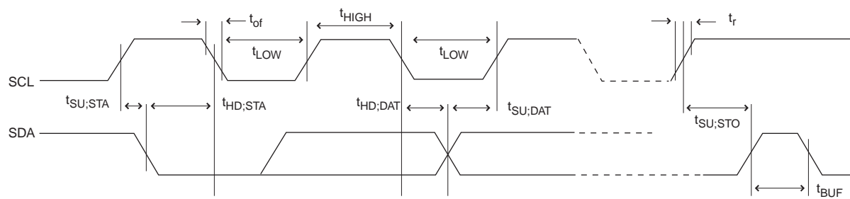
Figure 46-31. Two-wire Serial Bus Timing
