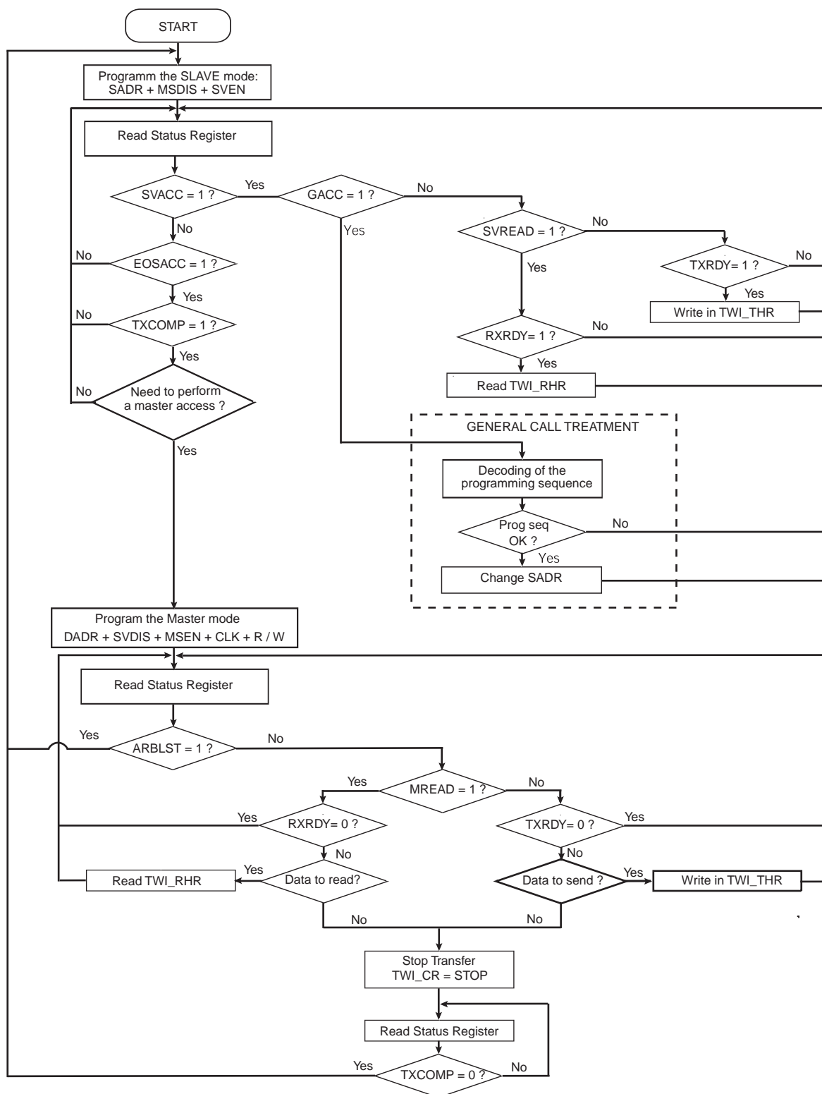
Figure 37-24. Multi-master Flowchart
