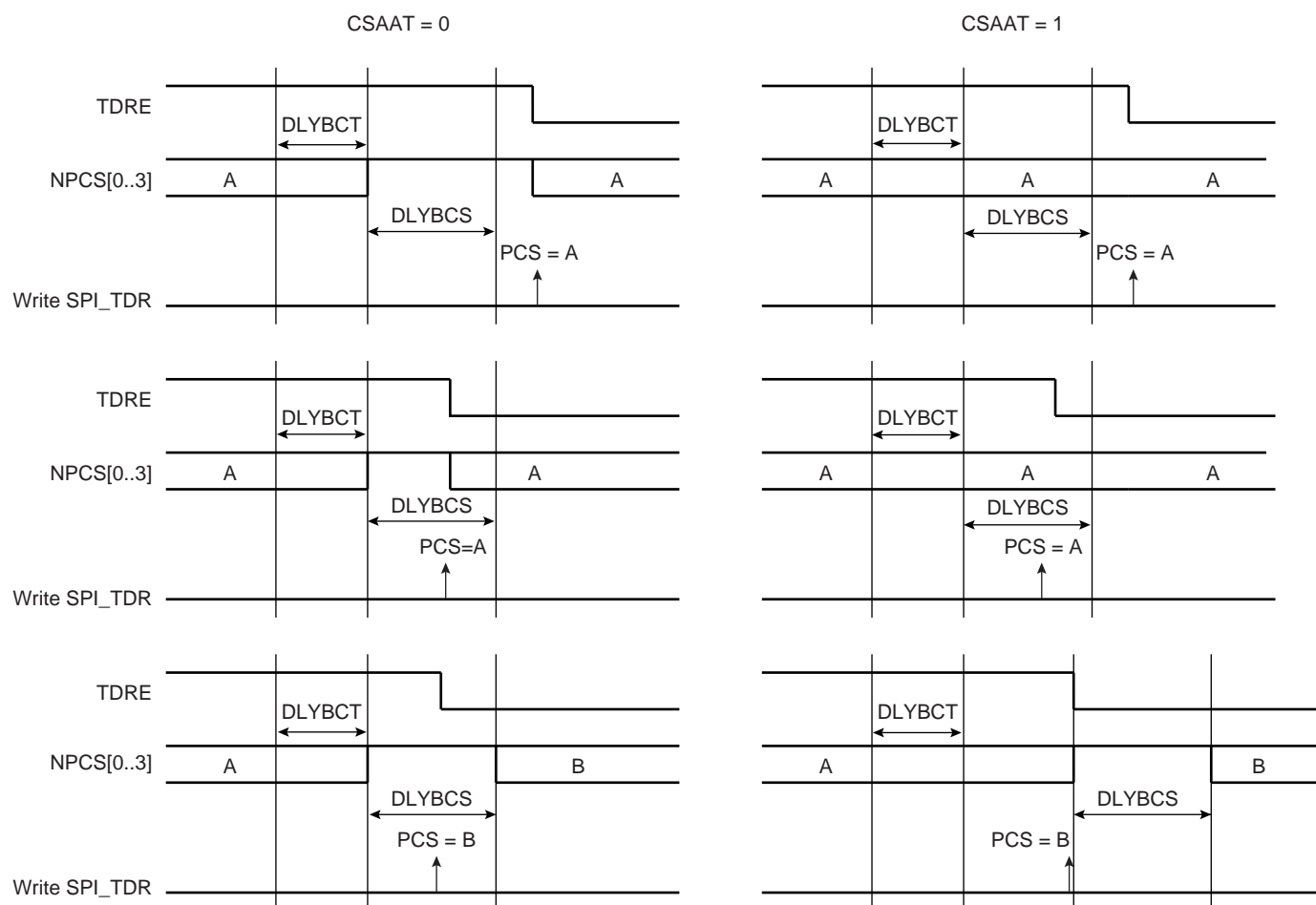
Figure 35-10. Peripheral Deselection
