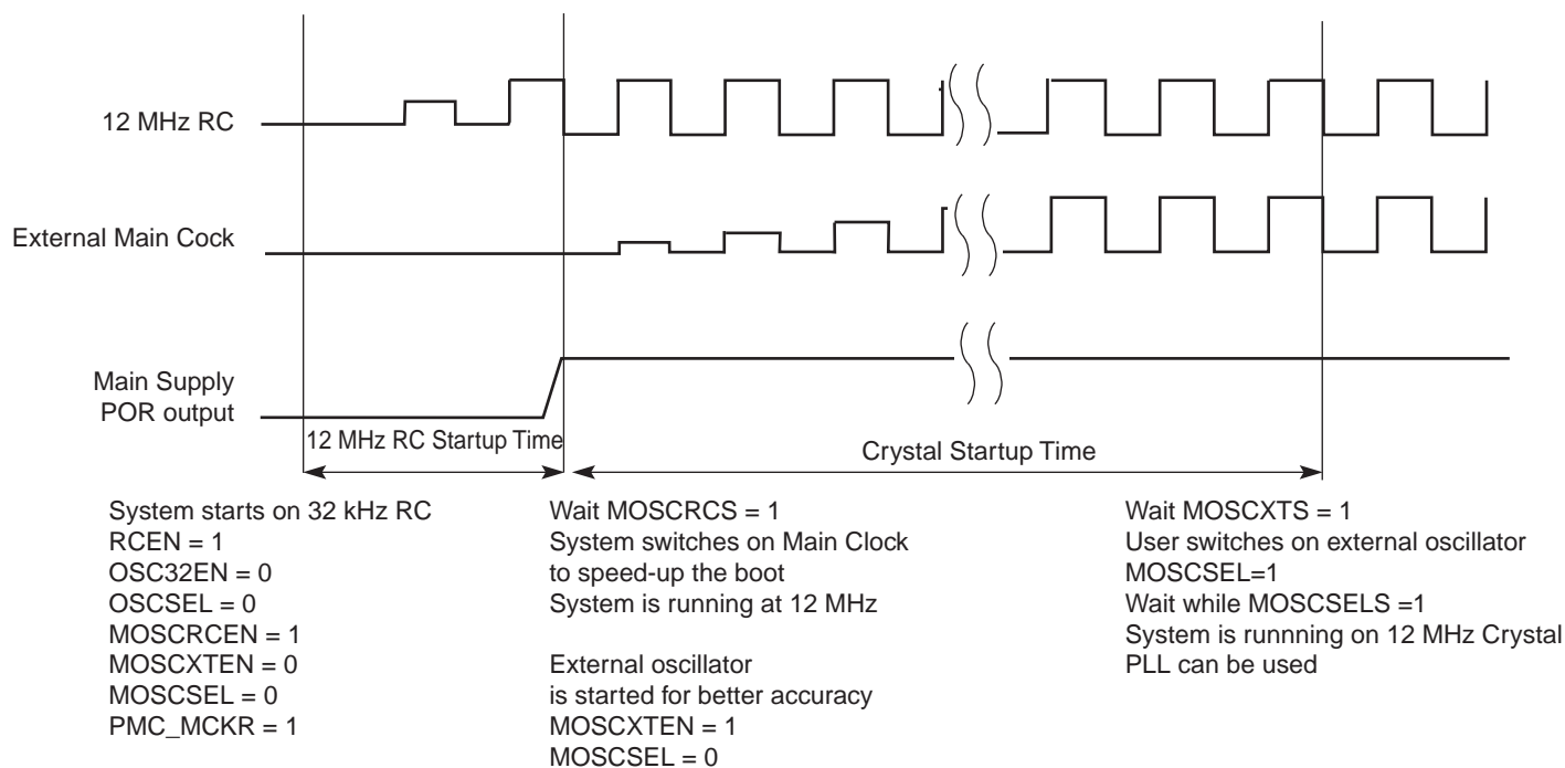
Figure 21-5. PMC Startup
