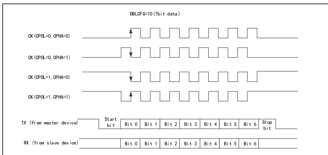
Figure 96 USART Synchronous Transmission Timing Diagram (DBLCFG=10)
