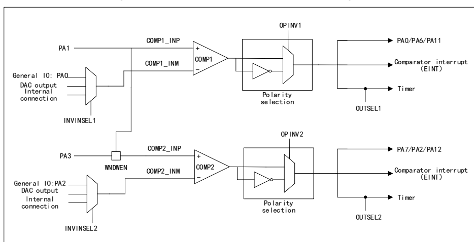
Figure 140 COMP Structure Block Diagram
