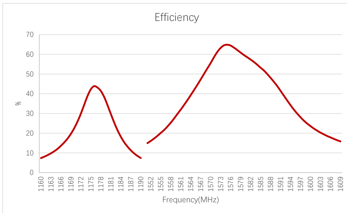
Efficiency (%)
