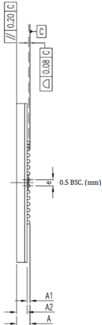
Figure 7-2 Side View
