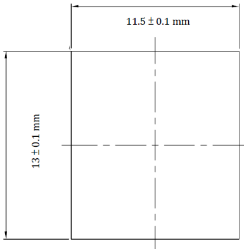
Figure 7-1 Top View
