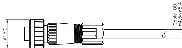
A size connector, field installable cable lock bayonet, female socket female pin, solder bucket
