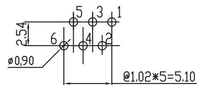
PCB LAYOUT - COMPONENT VIEW
