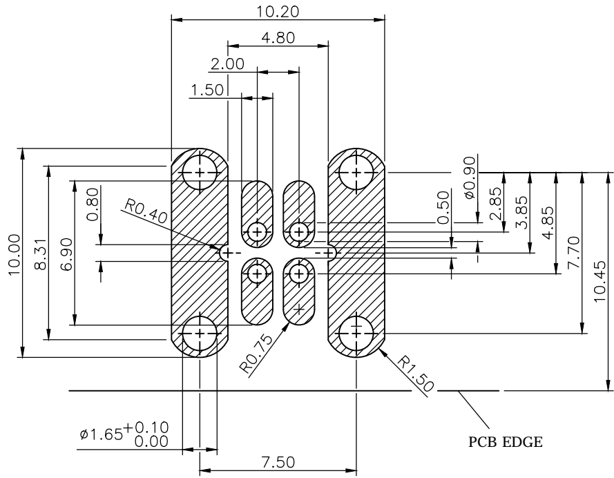
Recommended Layout (top view) General Tolerance: \pm 0.05\text{mm}
