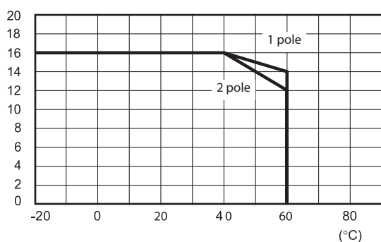
L 12 - Rated current v ambient temperature
