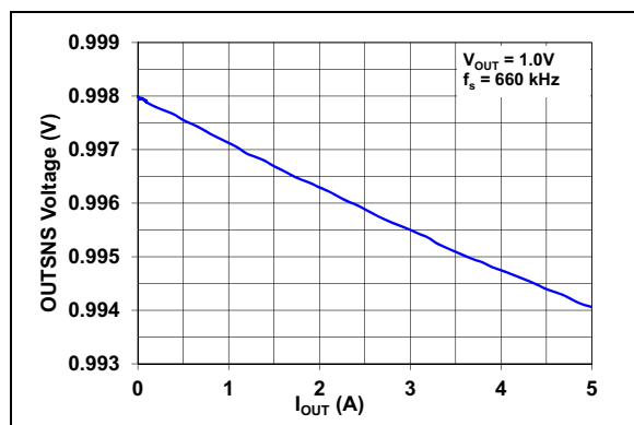
FIGURE 2-19: Load Regulation: OUTSNS Voltage vs. I_{OUT} .
