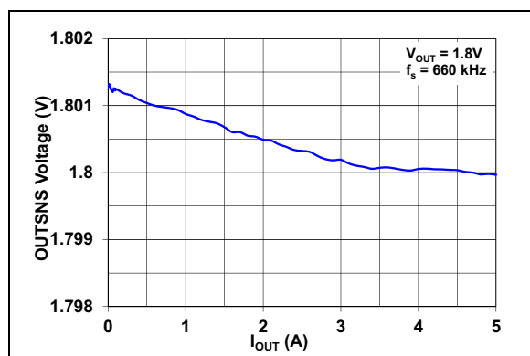
FIGURE 2-20: Load Regulation: OUTSNS Voltage vs. I_{OUT} .
