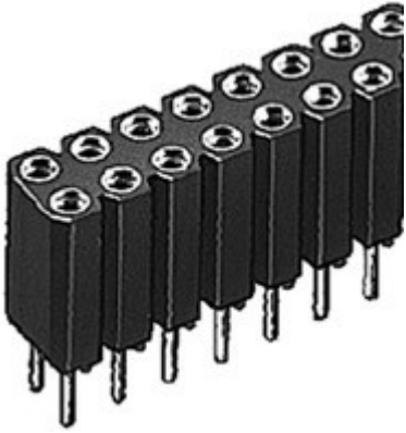
PCB connectors > Female headers inner contact spring surface: Ni + 0.75µm Au
