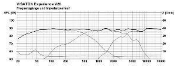
Frequency response
