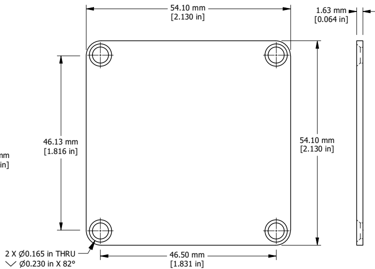
END PLATE
