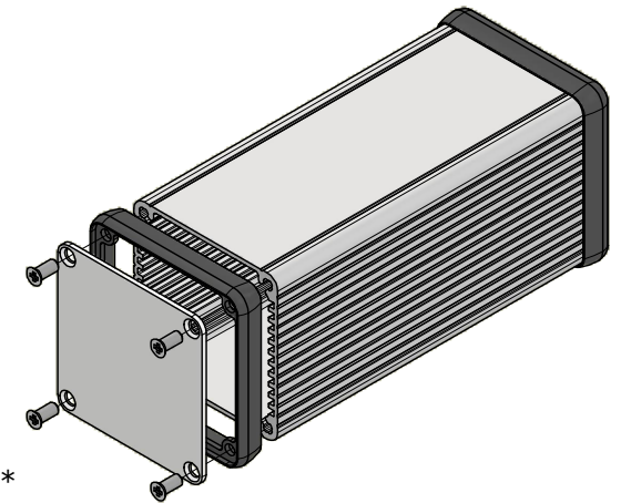
ISOMETRIC VIEW
