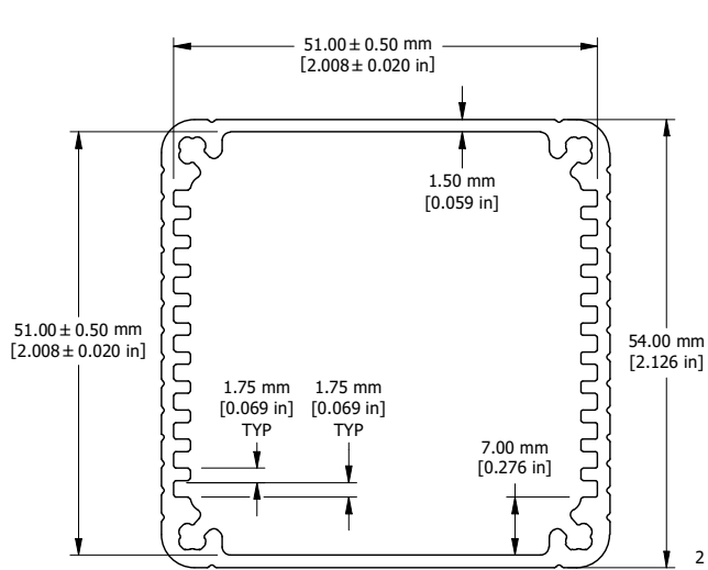
EXTRUSION
