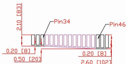
Detail C
