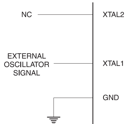
Figure 11-4. External Clock Drive Configuration
