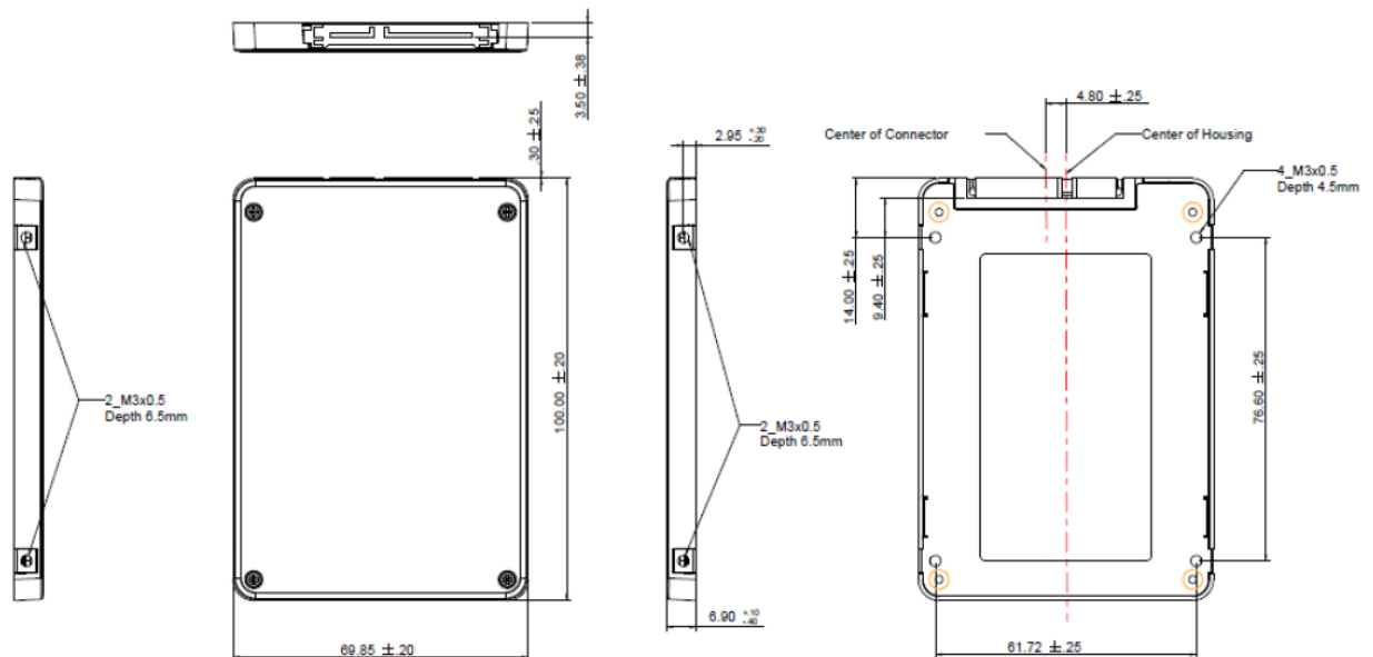
Figure 7-2 Physical Dimensions
