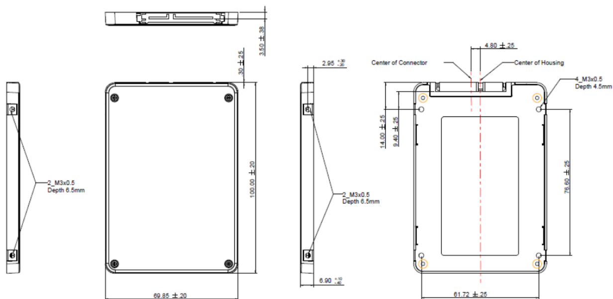
Figure 7-1 Physical Dimensions
