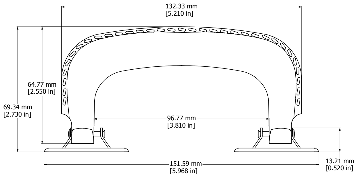
FRONT VIEW
