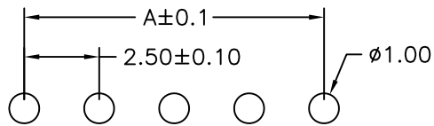
Recommand PCB Layout
