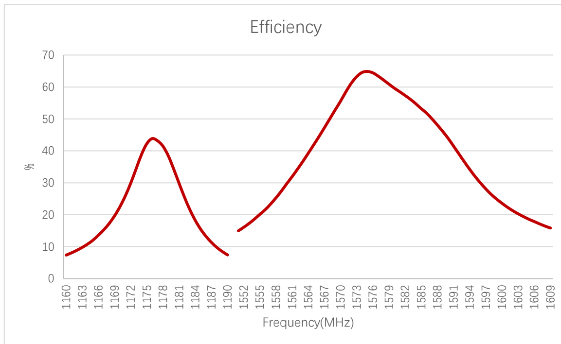
Efficiency (%)
