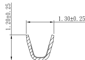
B-B SECTION ( WIRE BARREL )
