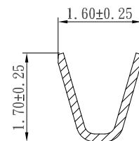
A-A SECTION ( INSULATION BARREL )
